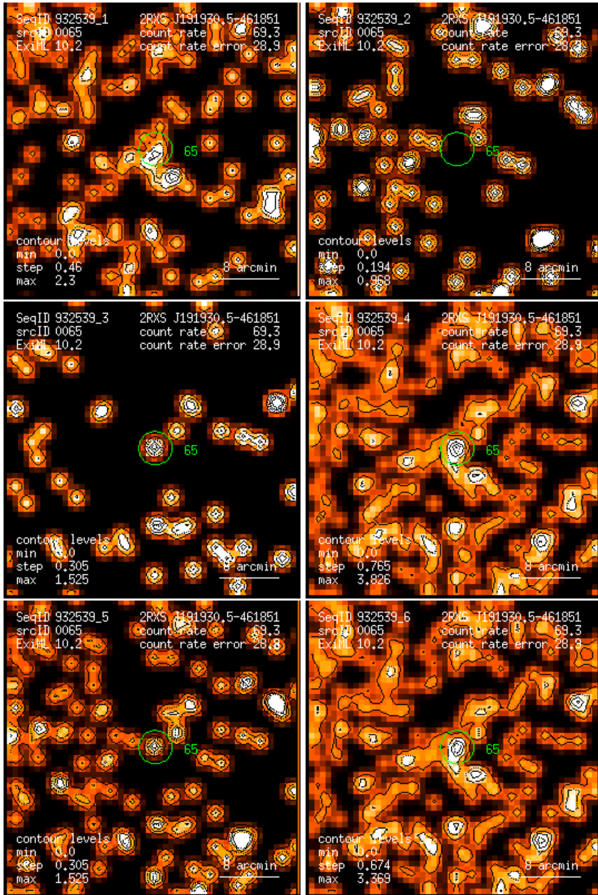
Figure 65: RASS 932539: detection 0065: band rate images, Gaussian filter: (1) PSPC channels 11 – 41, (2) 52 – 90, (3) 91 – 201, (4) 11 – 235, (5) 52 – 201, (6) 11 – 201. Broad band rates in counts/ks. Band rate contour levels in counts/ks/arcmin 2 .
