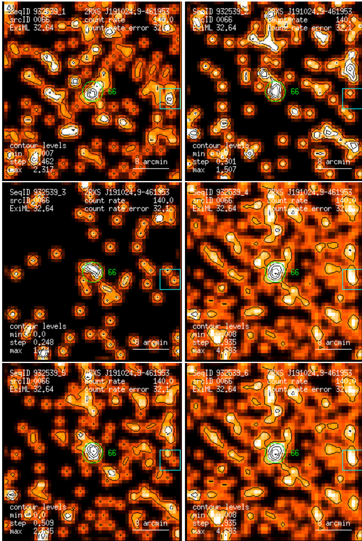
Figure 66: RASS 932539: detection 0066: band rate images, Gaussian filter: (1) PSPC channels 11 – 41, (2) 52 – 90, (3) 91 – 201, (4) 11 – 235, (5) 52 – 201, (6) 11 – 201. Broad band rates in counts/ks. Band rate contour levels in counts/ks/arcmin 2 .
