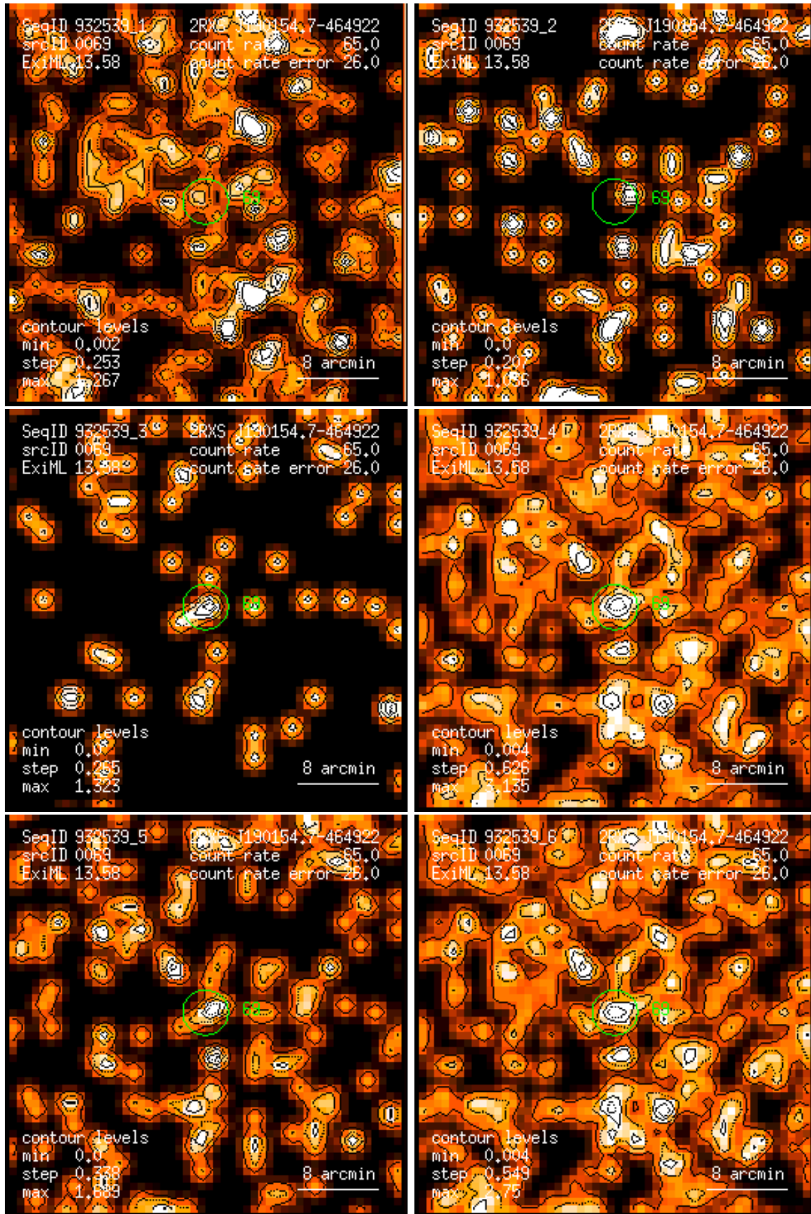
Figure 69: RASS 932539: detection 0069: band rate images, Gaussian filter: (1) PSPC channels 11 – 41, (2) 52 – 90, (3) 91 – 201, (4) 11 – 235, (5) 52 – 201, (6) 11 – 201. Broad band rates in counts/ks. Band rate contour levels in counts/ks/arcmin 2 .
