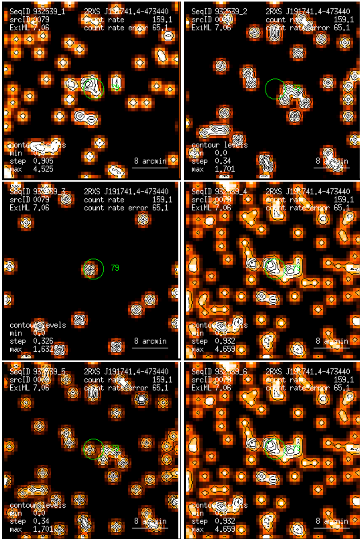
Figure 79: RASS 932539: detection 0079: band rate images, Gaussian filter: (1) PSPC channels 11 – 41, (2) 52 – 90, (3) 91 – 201, (4) 11 – 235, (5) 52 – 201, (6) 11 – 201. Broad band rates in counts/ks. Band rate contour levels in counts/ks/arcmin 2 .
