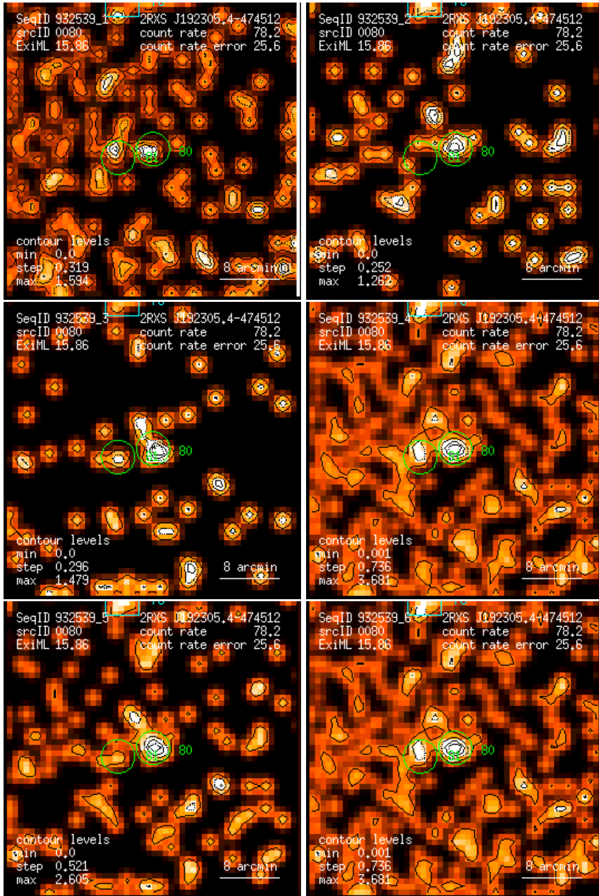
Figure 80: RASS 932539: detection 0080: band rate images, Gaussian filter: (1) PSPC channels 11 – 41, (2) 52 – 90, (3) 91 – 201, (4) 11 – 235, (5) 52 – 201, (6) 11 – 201. Broad band rates in counts/ks. Band rate contour levels in counts/ks/arcmin 2 .
