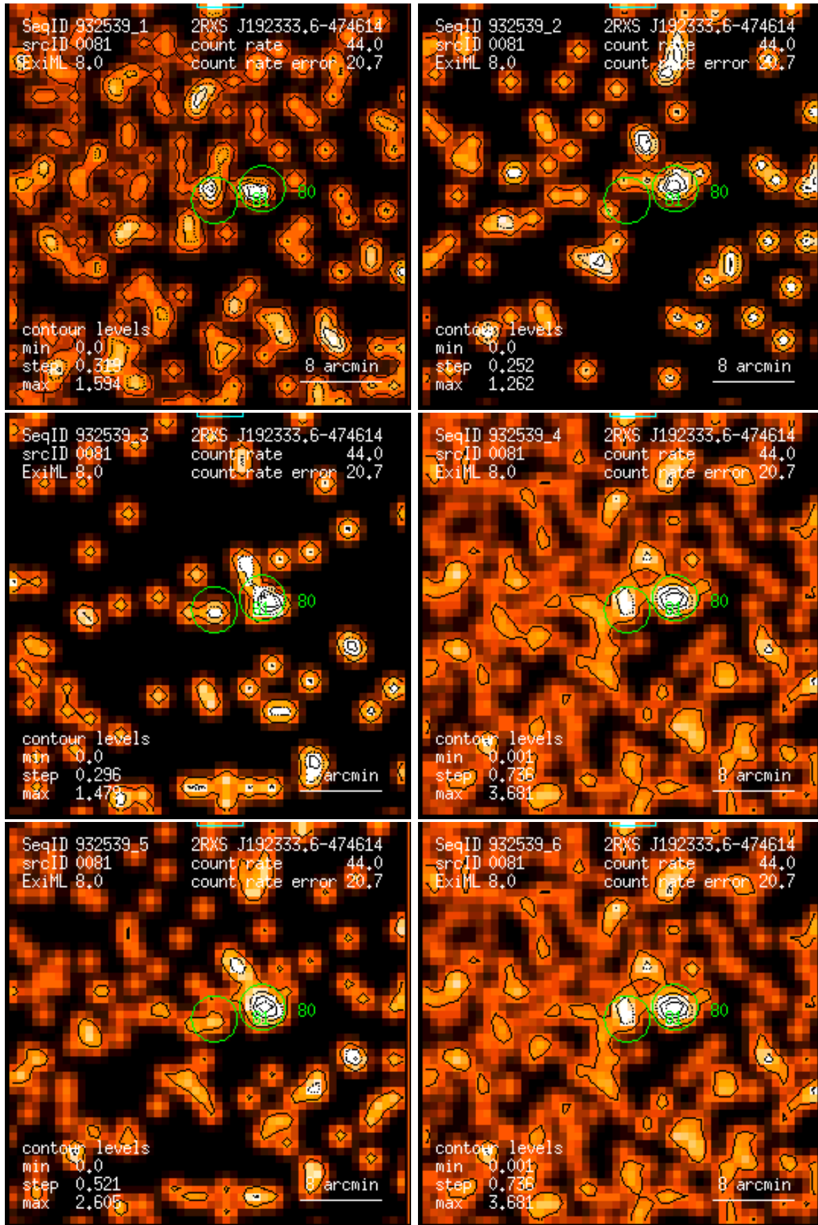
Figure 81: RASS 932539: detection 0081: band rate images, Gaussian filter: (1) PSPC channels 11 – 41, (2) 52 – 90, (3) 91 – 201, (4) 11 – 235, (5) 52 – 201, (6) 11 – 201. Broad band rates in counts/ks. Band rate contour levels in counts/ks/arcmin 2 .
