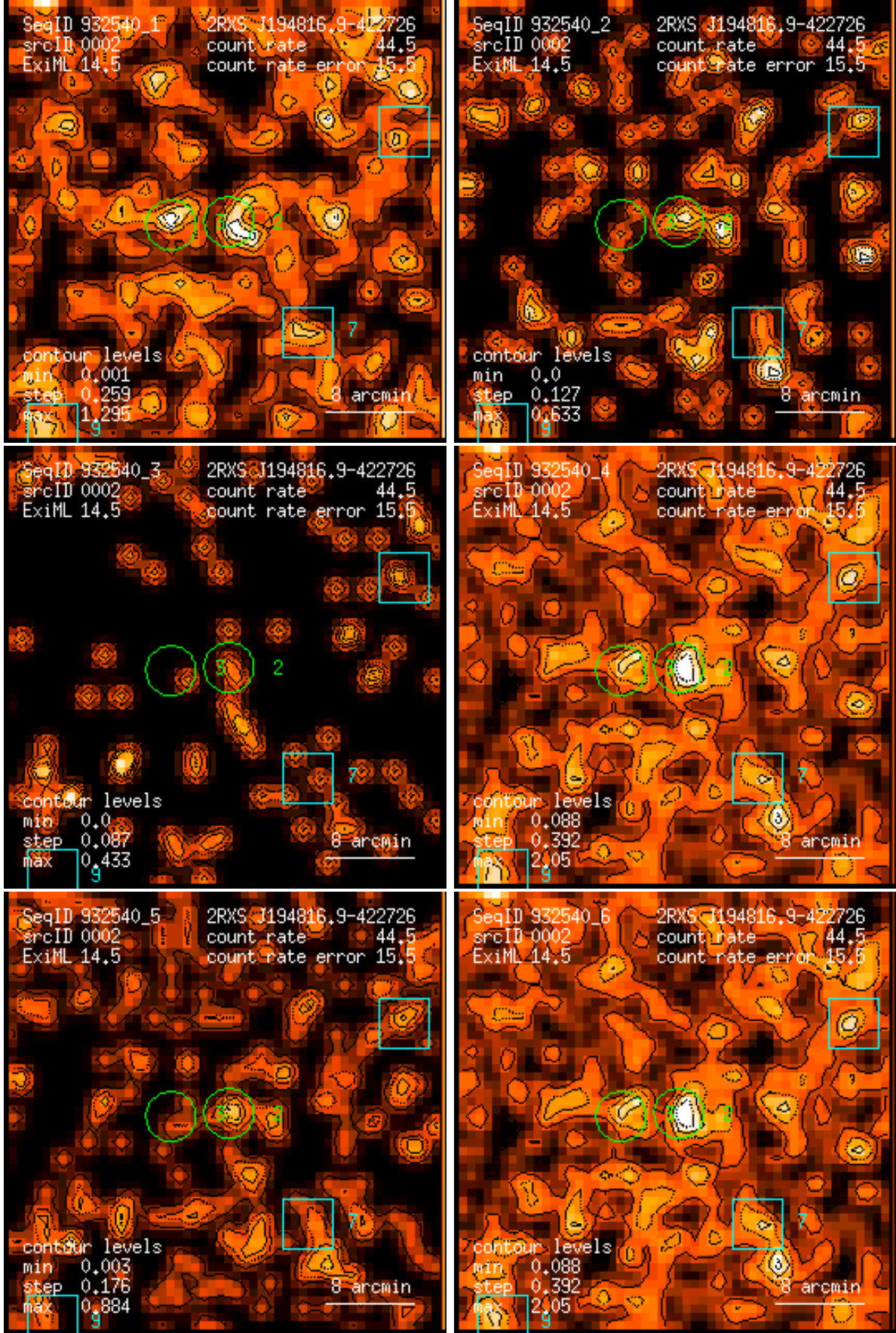
Figure 2: RASS 932540: detection 0002: band rate images, Gaussian filter: (1) PSPC channels 11 – 41, (2) 52 – 90, (3) 91 – 201, (4) 11 – 235, (5) 52 – 201, (6) 11 – 201. Broad band rates in counts/ks. Band rate contour levels in counts/ks/arcmin 2 .
