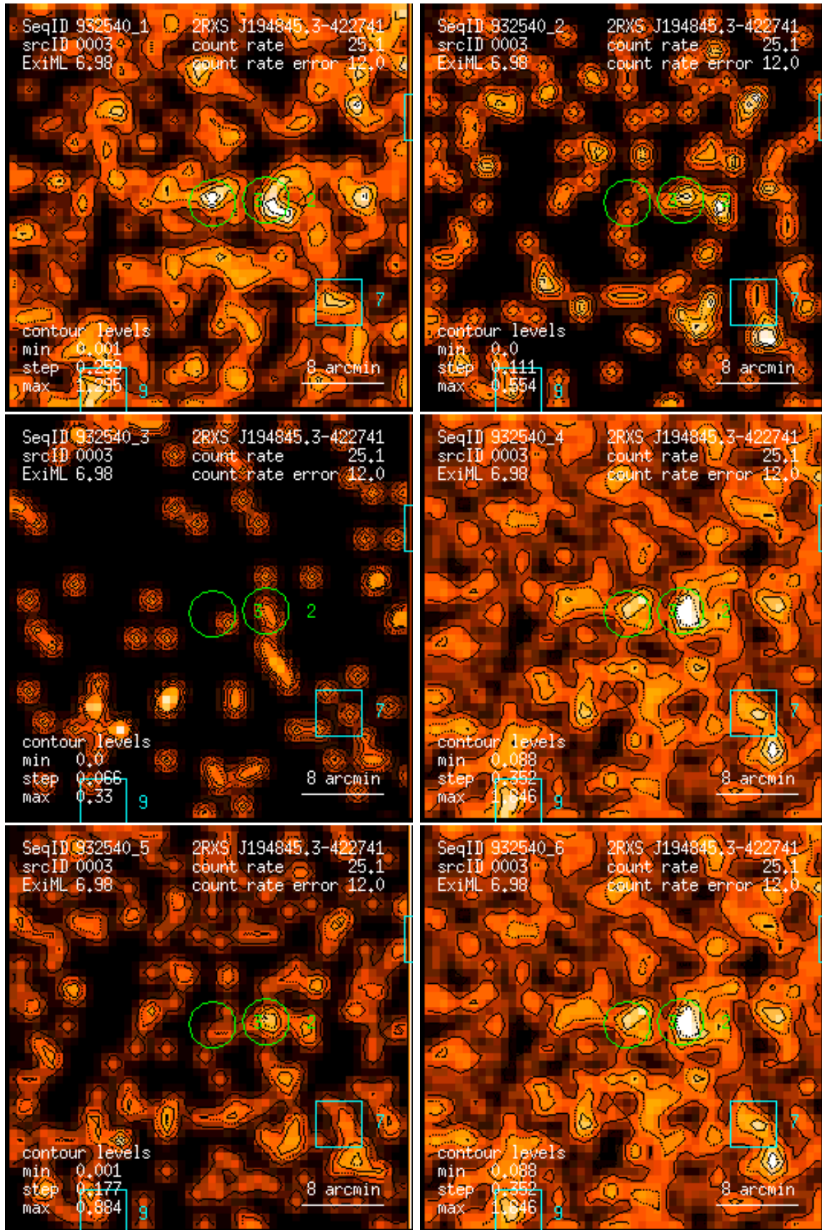
Figure 3: RASS 932540: detection 0003: band rate images, Gaussian filter: (1) PSPC channels 11 – 41, (2) 52 – 90, (3) 91 – 201, (4) 11 – 235, (5) 52 – 201, (6) 11 – 201. Broad band rates in counts/ks. Band rate contour levels in counts/ks/arcmin 2 .
