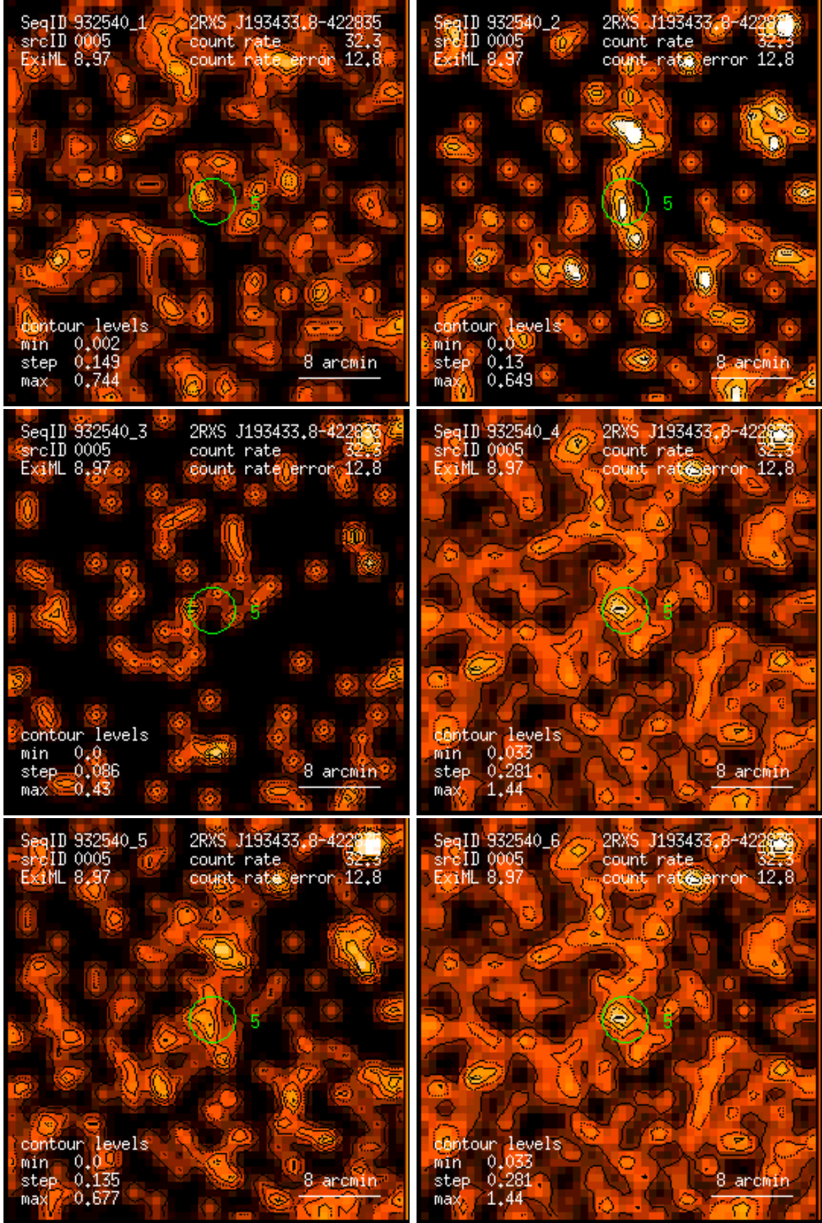
Figure 5: RASS 932540: detection 0005: band rate images, Gaussian filter: (1) PSPC channels 11 – 41, (2) 52 – 90, (3) 91 – 201, (4) 11 – 235, (5) 52 – 201, (6) 11 – 201. Broad band rates in counts/ks. Band rate contour levels in counts/ks/arcmin 2 .
