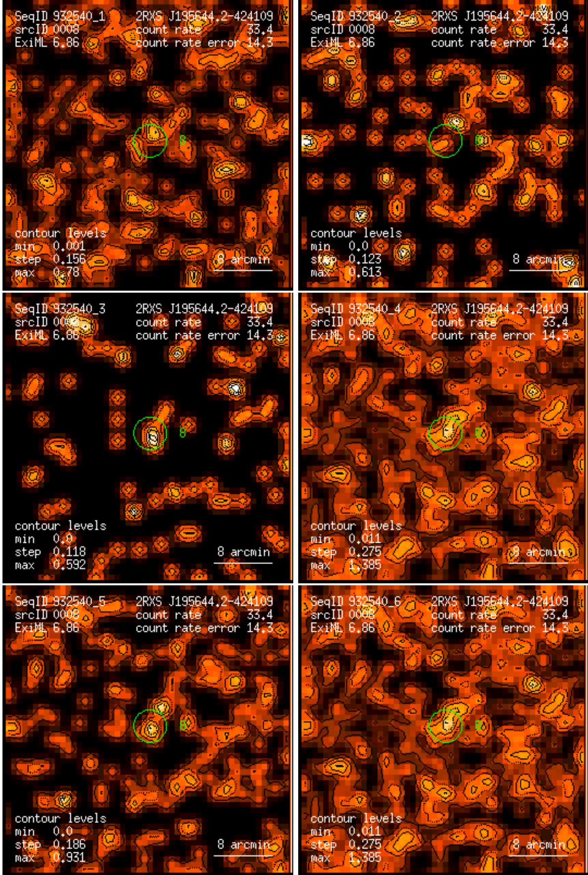
Figure 8: RASS 932540: detection 0008: band rate images, Gaussian filter: (1) PSPC channels 11 – 41, (2) 52 – 90, (3) 91 – 201, (4) 11 – 235, (5) 52 – 201, (6) 11 – 201. Broad band rates in counts/ks. Band rate contour levels in counts/ks/arcmin 2 .
