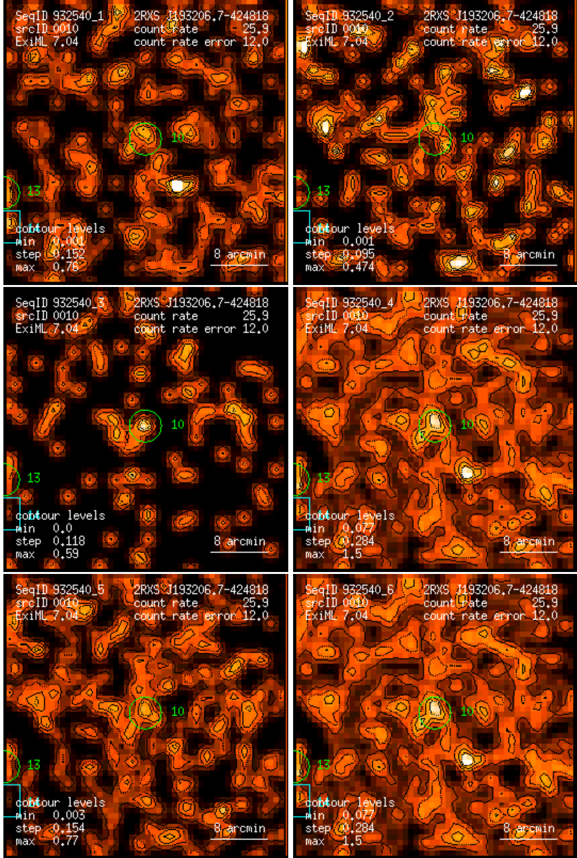
Figure 10: RASS 932540: detection 0010: band rate images, Gaussian filter: (1) PSPC channels 11 – 41, (2) 52 – 90, (3) 91 – 201, (4) 11 – 235, (5) 52 – 201, (6) 11 – 201. Broad band rates in counts/ks. Band rate contour levels in counts/ks/arcmin 2 .
