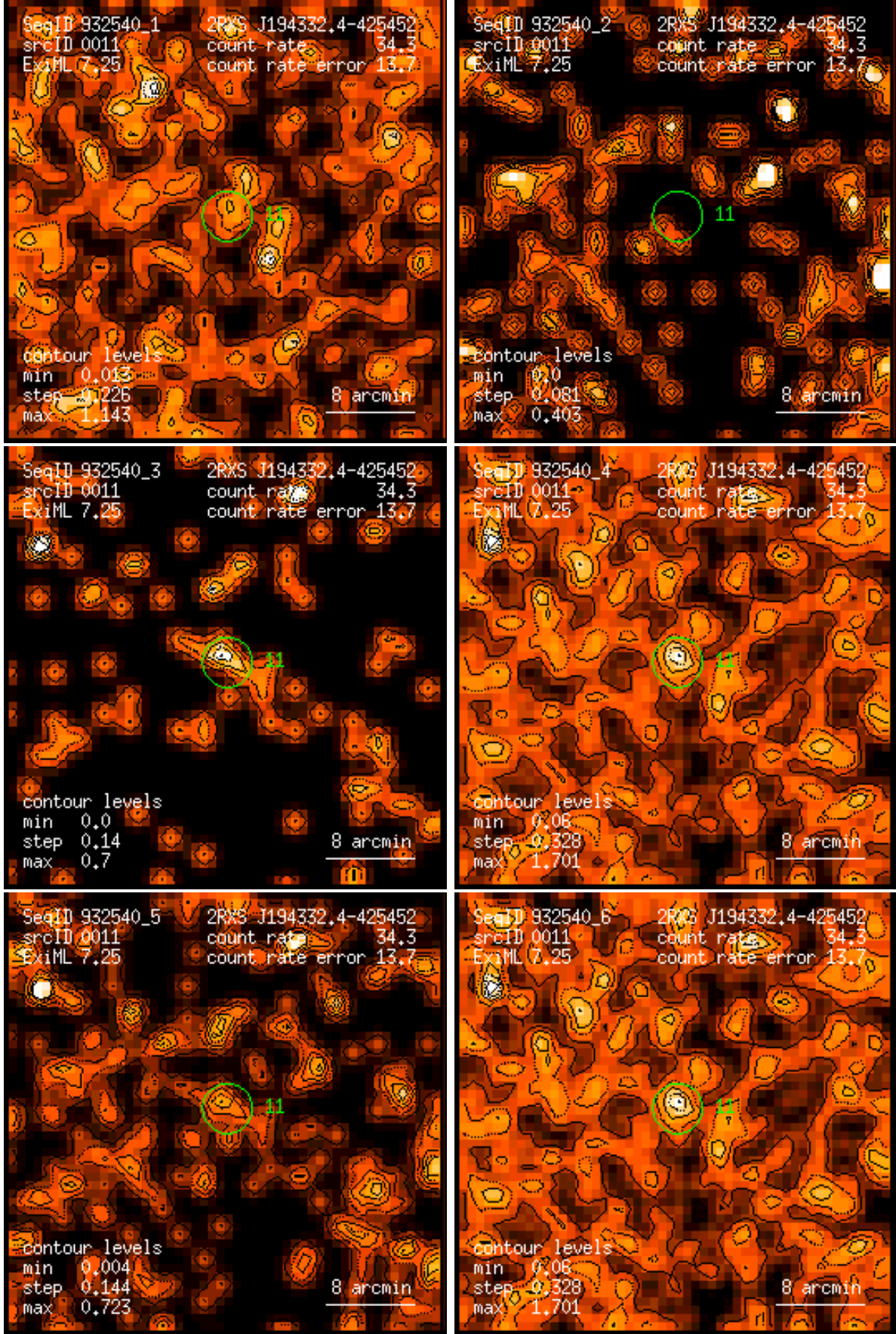
Figure 11: RASS 932540: detection 0011: band rate images, Gaussian filter: (1) PSPC channels 11 – 41, (2) 52 – 90, (3) 91 – 201, (4) 11 – 235, (5) 52 – 201, (6) 11 – 201. Broad band rates in counts/ks. Band rate contour levels in counts/ks/arcmin 2 .
