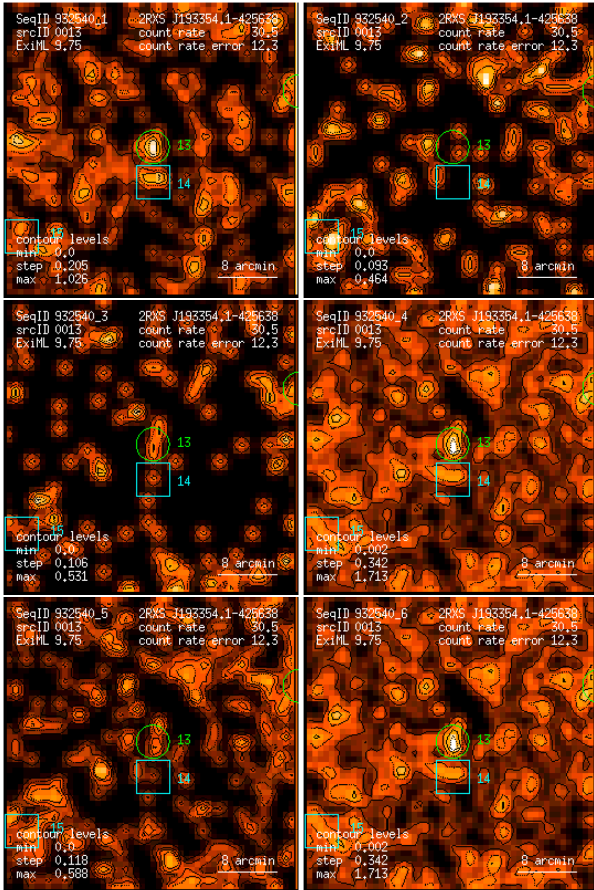
Figure 13: RASS 932540: detection 0013: band rate images, Gaussian filter: (1) PSPC channels 11 – 41, (2) 52 – 90, (3) 91 – 201, (4) 11 – 235, (5) 52 – 201, (6) 11 – 201. Broad band rates in counts/ks. Band rate contour levels in counts/ks/arcmin 2 .
