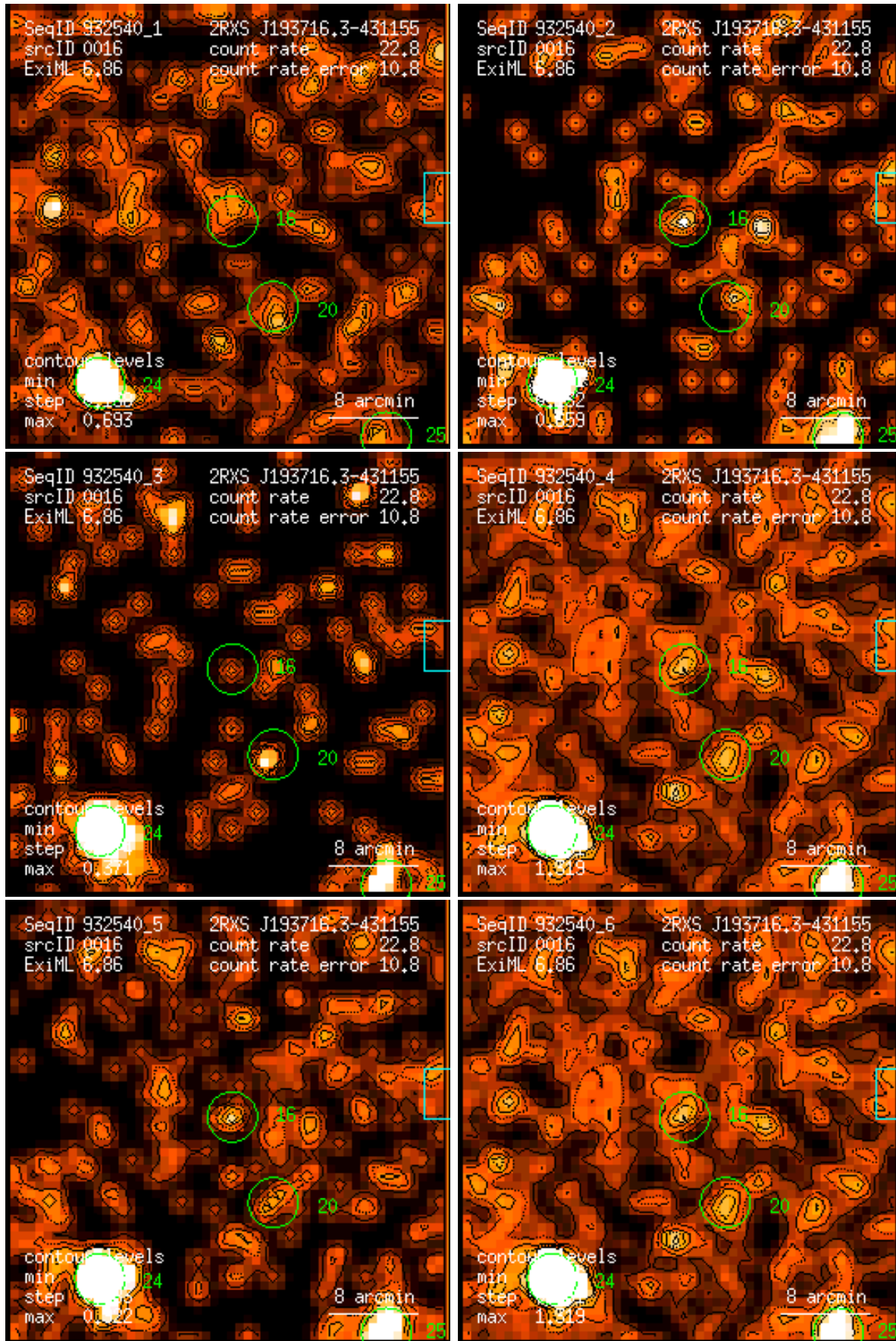
Figure 16: RASS 932540: detection 0016: band rate images, Gaussian filter: (1) PSPC channels 11 – 41, (2) 52 – 90, (3) 91 – 201, (4) 11 – 235, (5) 52 – 201, (6) 11 – 201. Broad band rates in counts/ks. Band rate contour levels in counts/ks/arcmin 2 .
