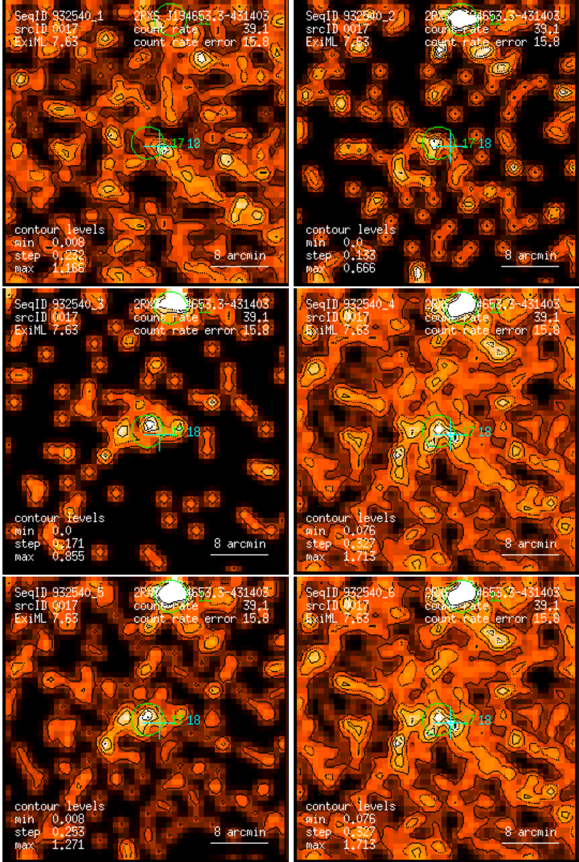
Figure 17: RASS 932540: detection 0017: band rate images, Gaussian filter: (1) PSPC channels 11 – 41, (2) 52 – 90, (3) 91 – 201, (4) 11 – 235, (5) 52 – 201, (6) 11 – 201. Broad band rates in counts/ks. Band rate contour levels in counts/ks/arcmin 2 .
