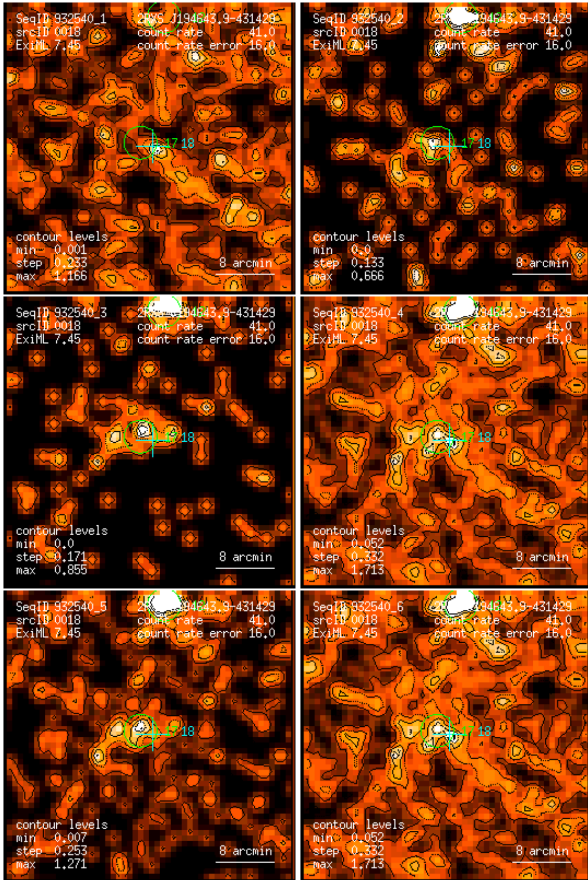
Figure 18: RASS 932540: detection 0018: band rate images, Gaussian filter: (1) PSPC channels 11 – 41, (2) 52 – 90, (3) 91 – 201, (4) 11 – 235, (5) 52 – 201, (6) 11 – 201. Broad band rates in counts/ks. Band rate contour levels in counts/ks/arcmin 2 .
