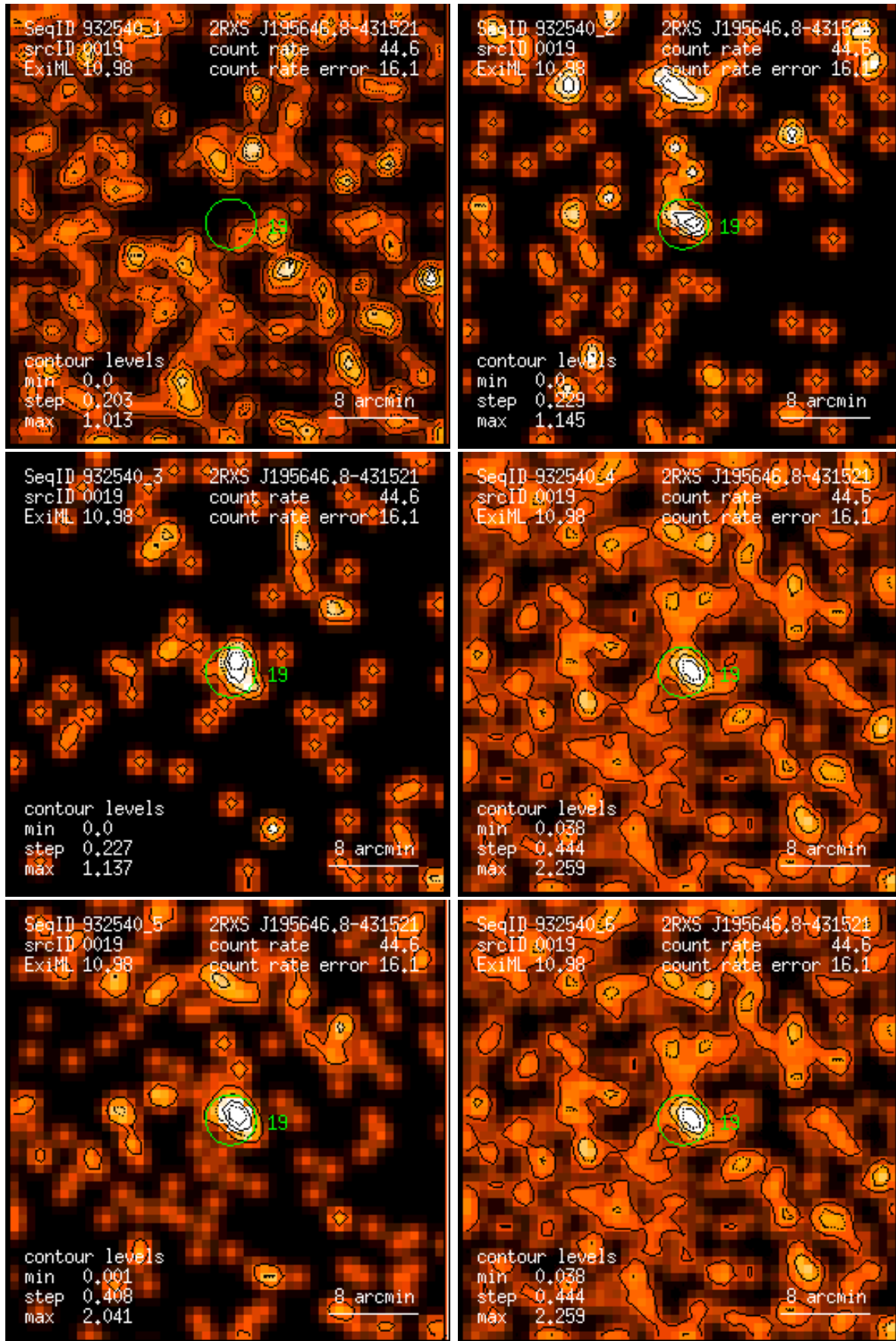
Figure 19: RASS 932540: detection 0019: band rate images, Gaussian filter: (1) PSPC channels 11 – 41, (2) 52 – 90, (3) 91 – 201, (4) 11 – 235, (5) 52 – 201, (6) 11 – 201. Broad band rates in counts/ks. Band rate contour levels in counts/ks/arcmin 2 .
