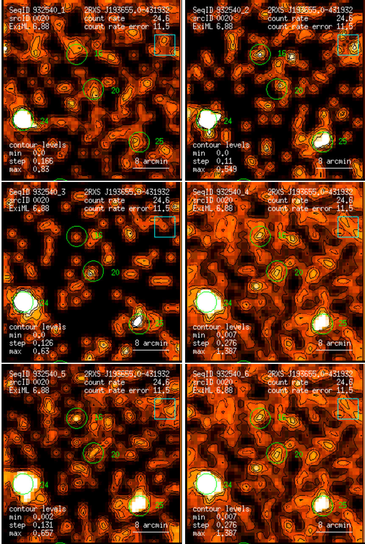
Figure 20: RASS 932540: detection 0020: band rate images, Gaussian filter: (1) PSPC channels 11 – 41, (2) 52 – 90, (3) 91 – 201, (4) 11 – 235, (5) 52 – 201, (6) 11 – 201. Broad band rates in counts/ks. Band rate contour levels in counts/ks/arcmin 2 .
