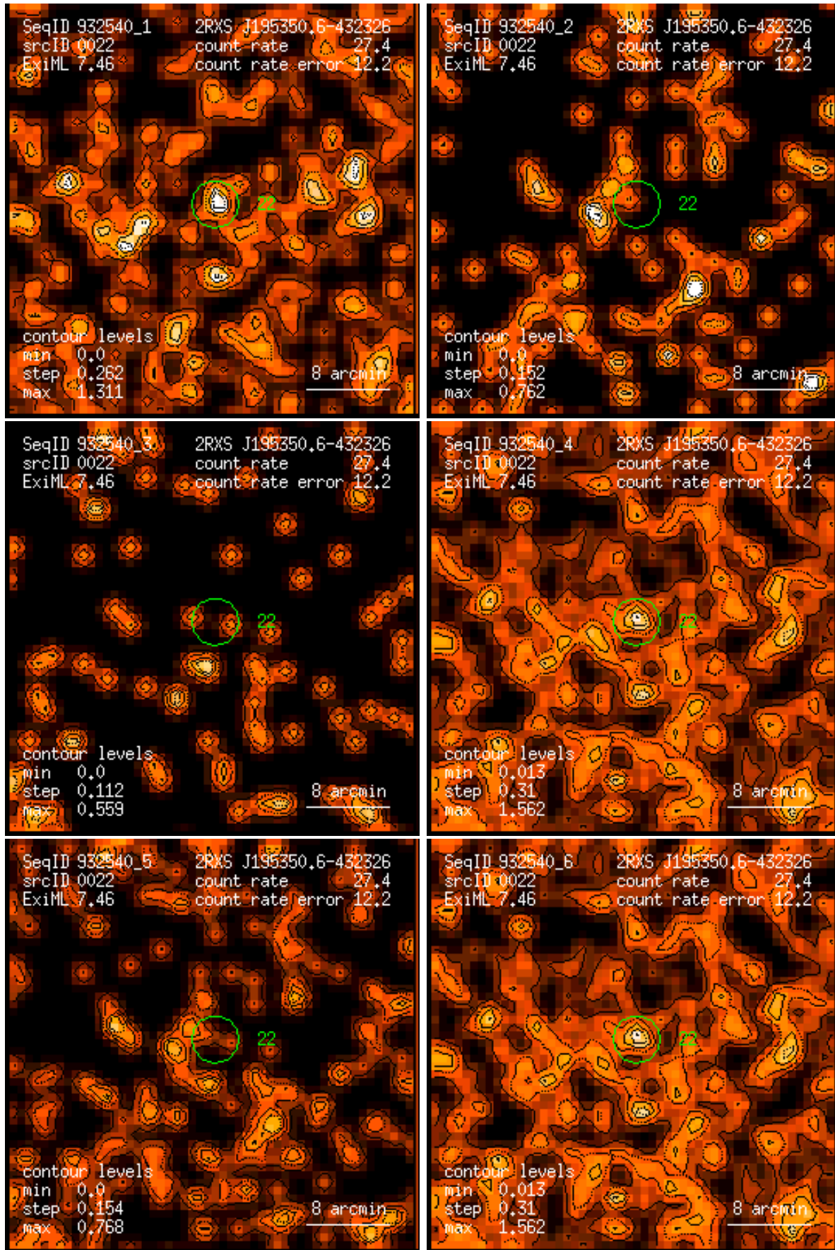
Figure 22: RASS 932540: detection 0022: band rate images, Gaussian filter: (1) PSPC channels 11 – 41, (2) 52 – 90, (3) 91 – 201, (4) 11 – 235, (5) 52 – 201, (6) 11 – 201. Broad band rates in counts/ks. Band rate contour levels in counts/ks/arcmin 2 .
