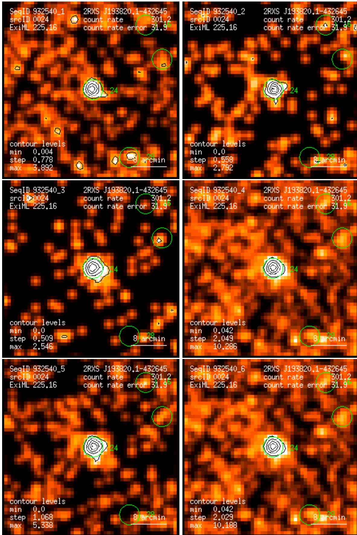
Figure 24: RASS 932540: detection 0024: band rate images, Gaussian filter: (1) PSPC channels 11 – 41, (2) 52 – 90, (3) 91 – 201, (4) 11 – 235, (5) 52 – 201, (6) 11 – 201. Broad band rates in counts/ks. Band rate contour levels in counts/ks/arcmin 2 .
