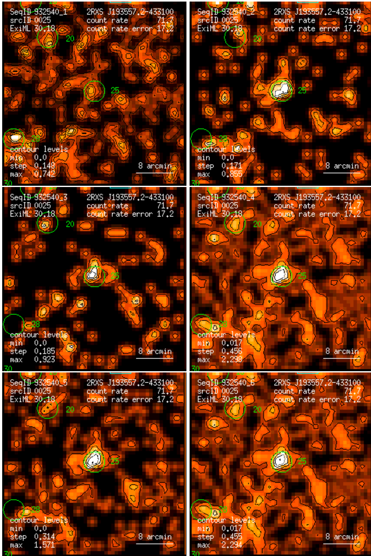
Figure 25: RASS 932540: detection 0025: band rate images, Gaussian filter: (1) PSPC channels 11 – 41, (2) 52 – 90, (3) 91 – 201, (4) 11 – 235, (5) 52 – 201, (6) 11 – 201. Broad band rates in counts/ks. Band rate contour levels in counts/ks/arcmin 2 .
