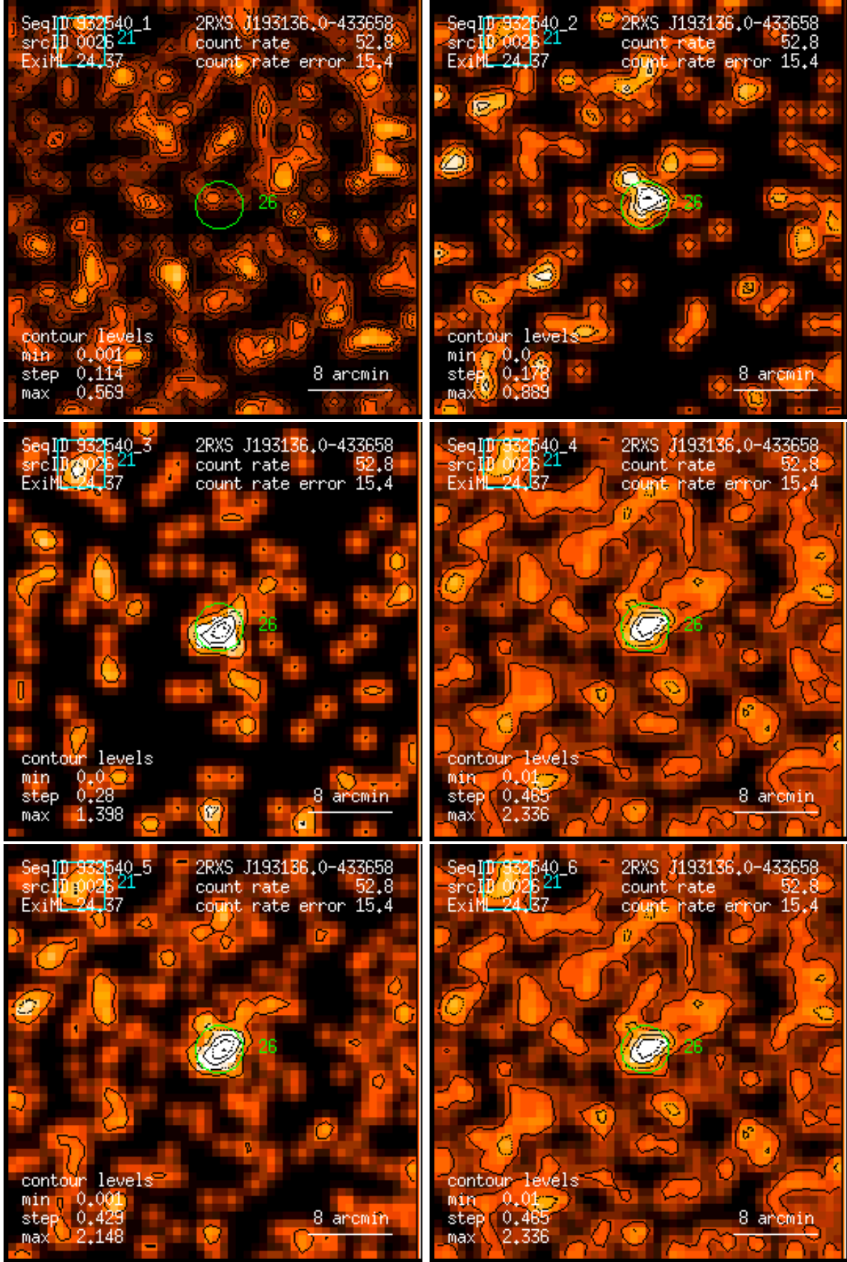
Figure 26: RASS 932540: detection 0026: band rate images, Gaussian filter: (1) PSPC channels 11 – 41, (2) 52 – 90, (3) 91 – 201, (4) 11 – 235, (5) 52 – 201, (6) 11 – 201. Broad band rates in counts/ks. Band rate contour levels in counts/ks/arcmin 2 .
