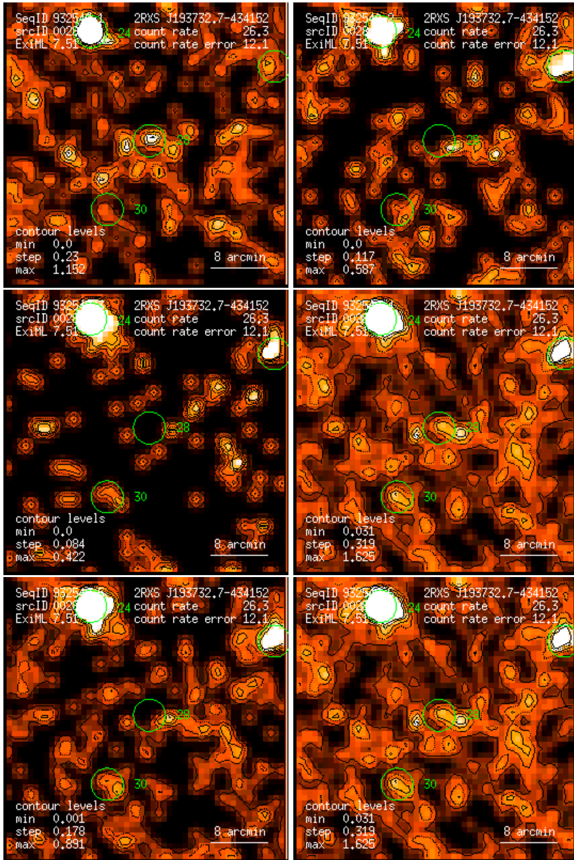
Figure 28: RASS 932540: detection 0028: band rate images, Gaussian filter: (1) PSPC channels 11 – 41, (2) 52 – 90, (3) 91 – 201, (4) 11 – 235, (5) 52 – 201, (6) 11 – 201. Broad band rates in counts/ks. Band rate contour levels in counts/ks/arcmin 2 .
