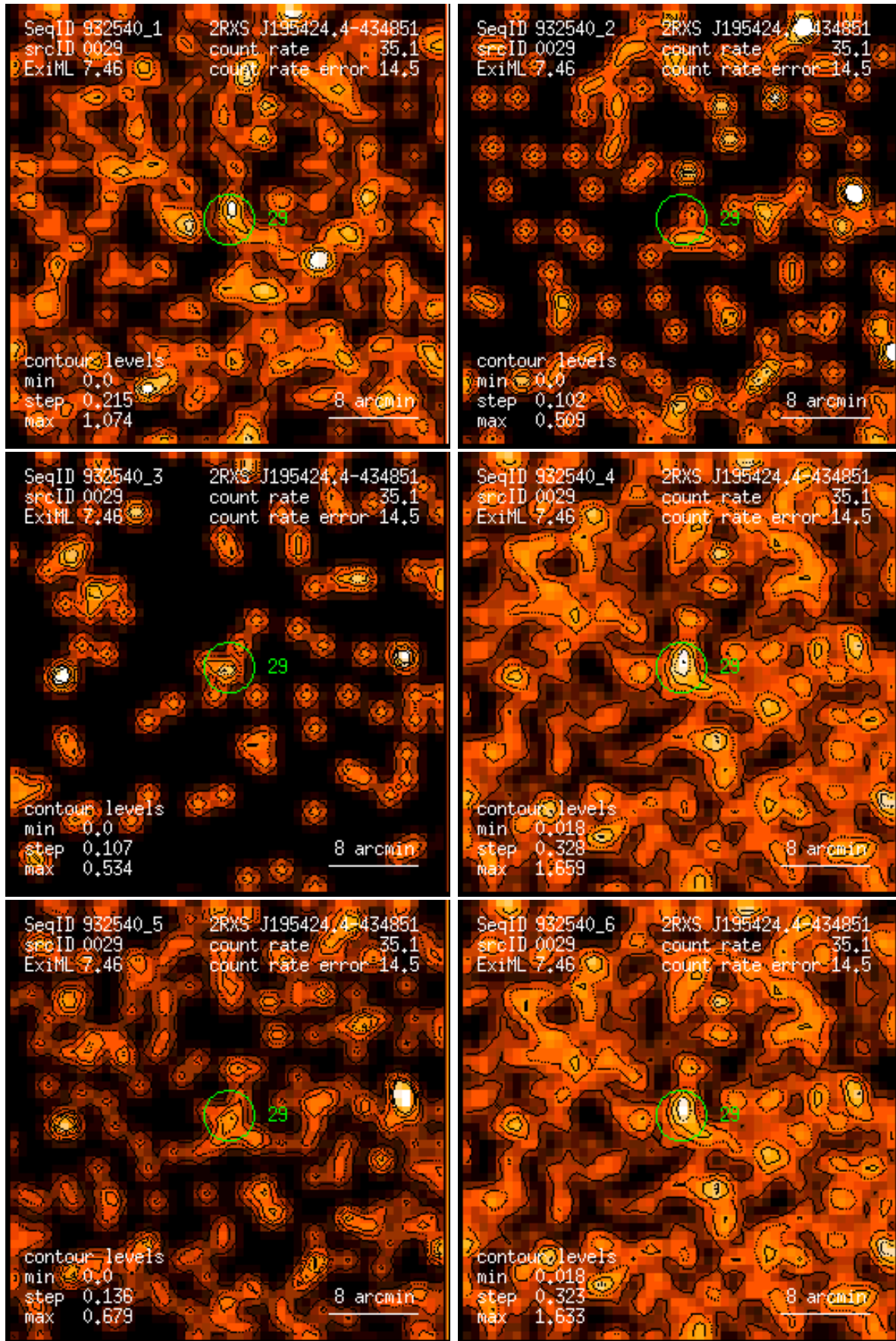
Figure 29: RASS 932540: detection 0029: band rate images, Gaussian filter: (1) PSPC channels 11 – 41, (2) 52 – 90, (3) 91 – 201, (4) 11 – 235, (5) 52 – 201, (6) 11 – 201. Broad band rates in counts/ks. Band rate contour levels in counts/ks/arcmin 2 .
