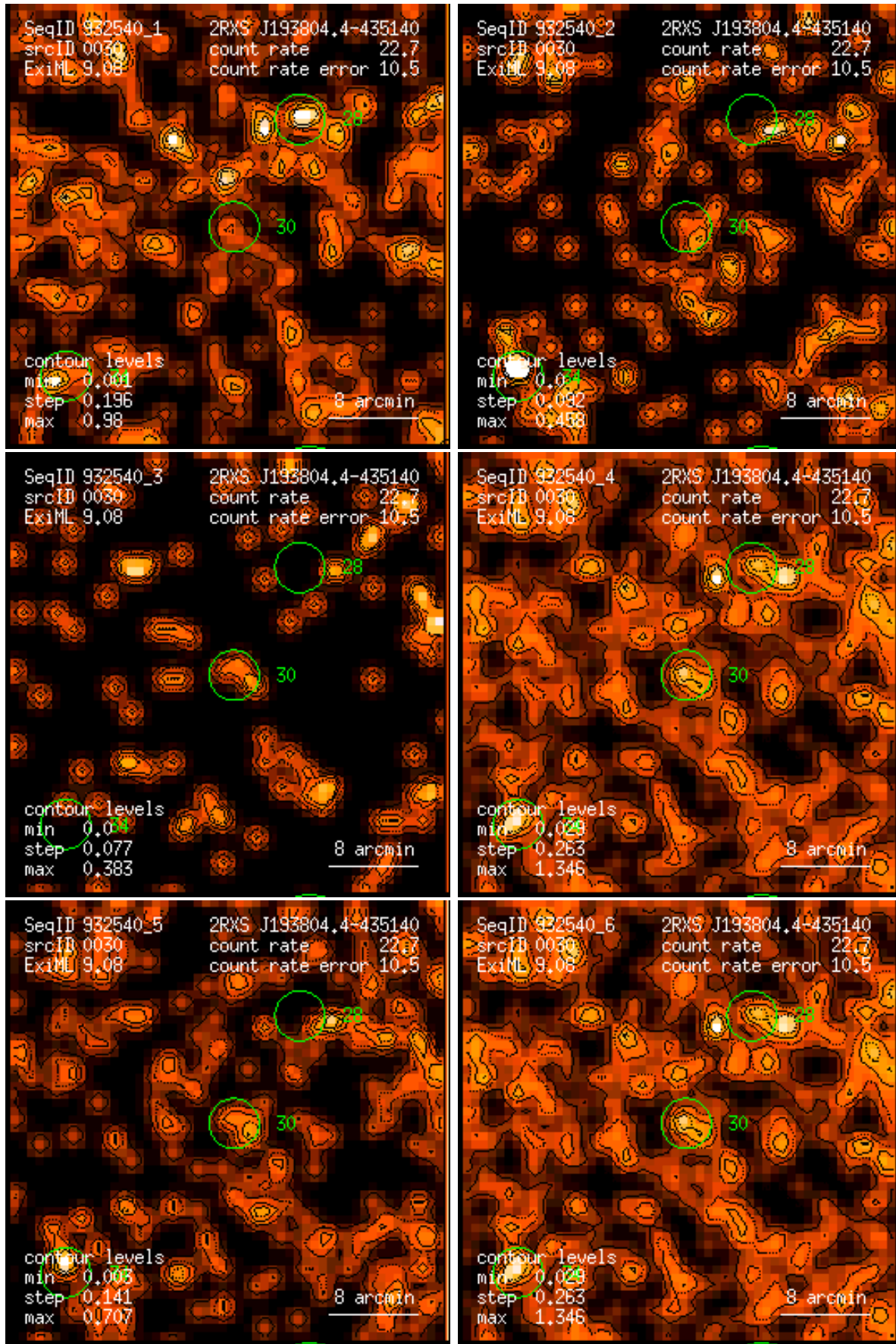
Figure 30: RASS 932540: detection 0030: band rate images, Gaussian filter: (1) PSPC channels 11 – 41, (2) 52 – 90, (3) 91 – 201, (4) 11 – 235, (5) 52 – 201, (6) 11 – 201. Broad band rates in counts/ks. Band rate contour levels in counts/ks/arcmin 2 .
