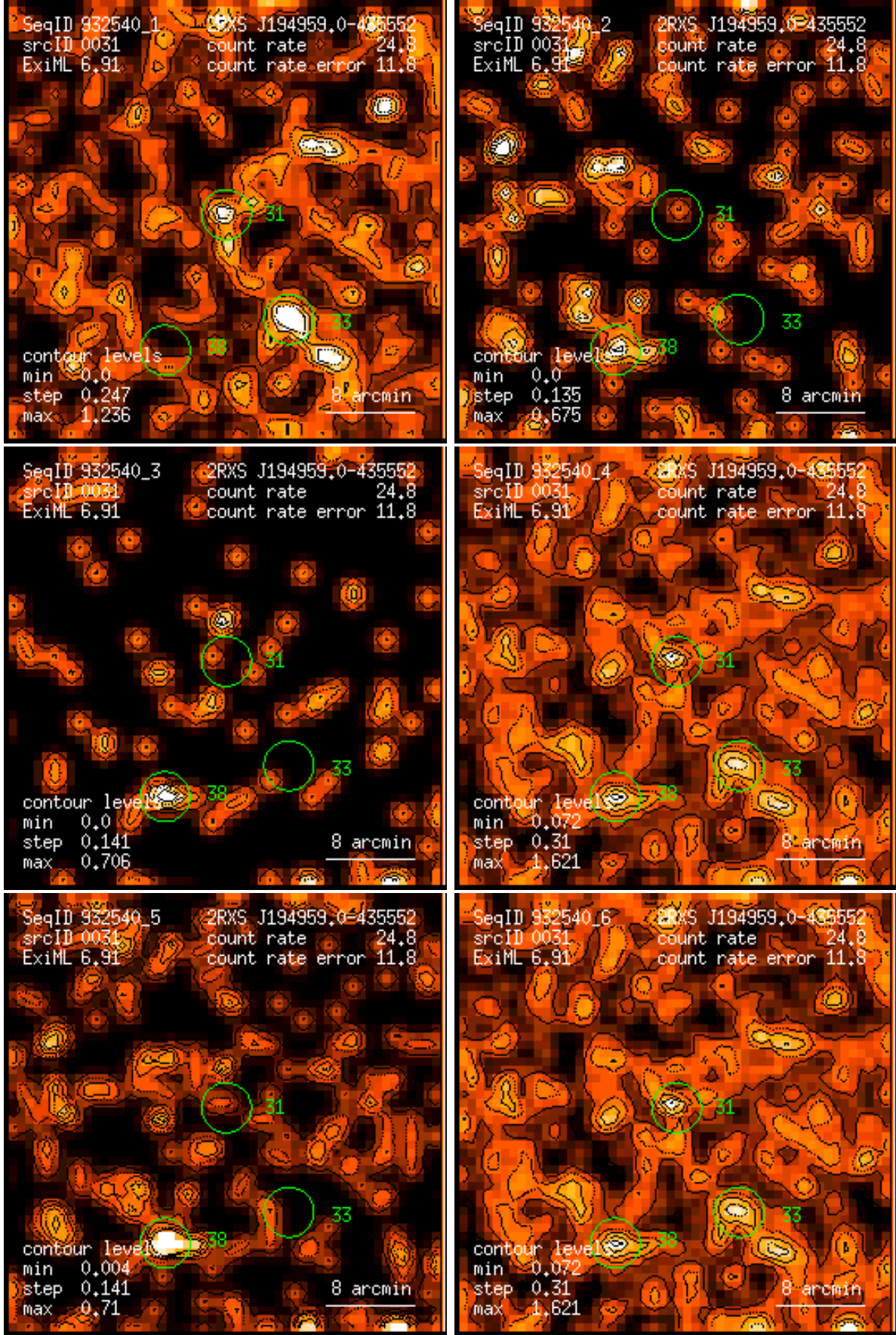
Figure 31: RASS 932540: detection 0031: band rate images, Gaussian filter: (1) PSPC channels 11 – 41, (2) 52 – 90, (3) 91 – 201, (4) 11 – 235, (5) 52 – 201, (6) 11 – 201. Broad band rates in counts/ks. Band rate contour levels in counts/ks/arcmin 2 .
