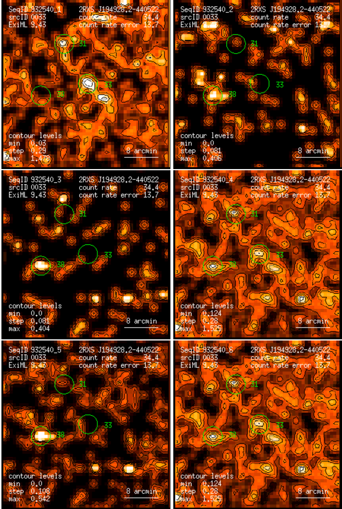
Figure 33: RASS 932540: detection 0033: band rate images, Gaussian filter: (1) PSPC channels 11 – 41, (2) 52 – 90, (3) 91 – 201, (4) 11 – 235, (5) 52 – 201, (6) 11 – 201. Broad band rates in counts/ks. Band rate contour levels in counts/ks/arcmin 2 .
