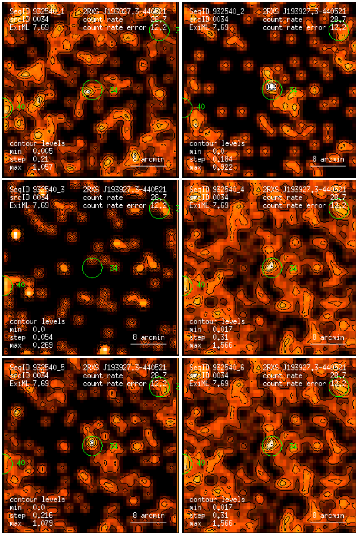
Figure 34: RASS 932540: detection 0034: band rate images, Gaussian filter: (1) PSPC channels 11 – 41, (2) 52 – 90, (3) 91 – 201, (4) 11 – 235, (5) 52 – 201, (6) 11 – 201. Broad band rates in counts/ks. Band rate contour levels in counts/ks/arcmin 2 .
