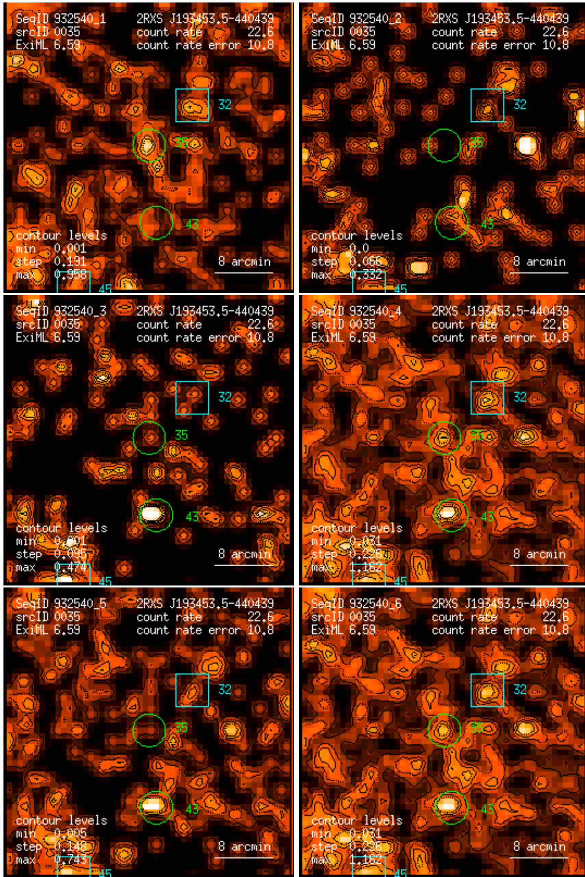
Figure 35: RASS 932540: detection 0035: band rate images, Gaussian filter: (1) PSPC channels 11 – 41, (2) 52 – 90, (3) 91 – 201, (4) 11 – 235, (5) 52 – 201, (6) 11 – 201. Broad band rates in counts/ks. Band rate contour levels in counts/ks/arcmin 2 .
