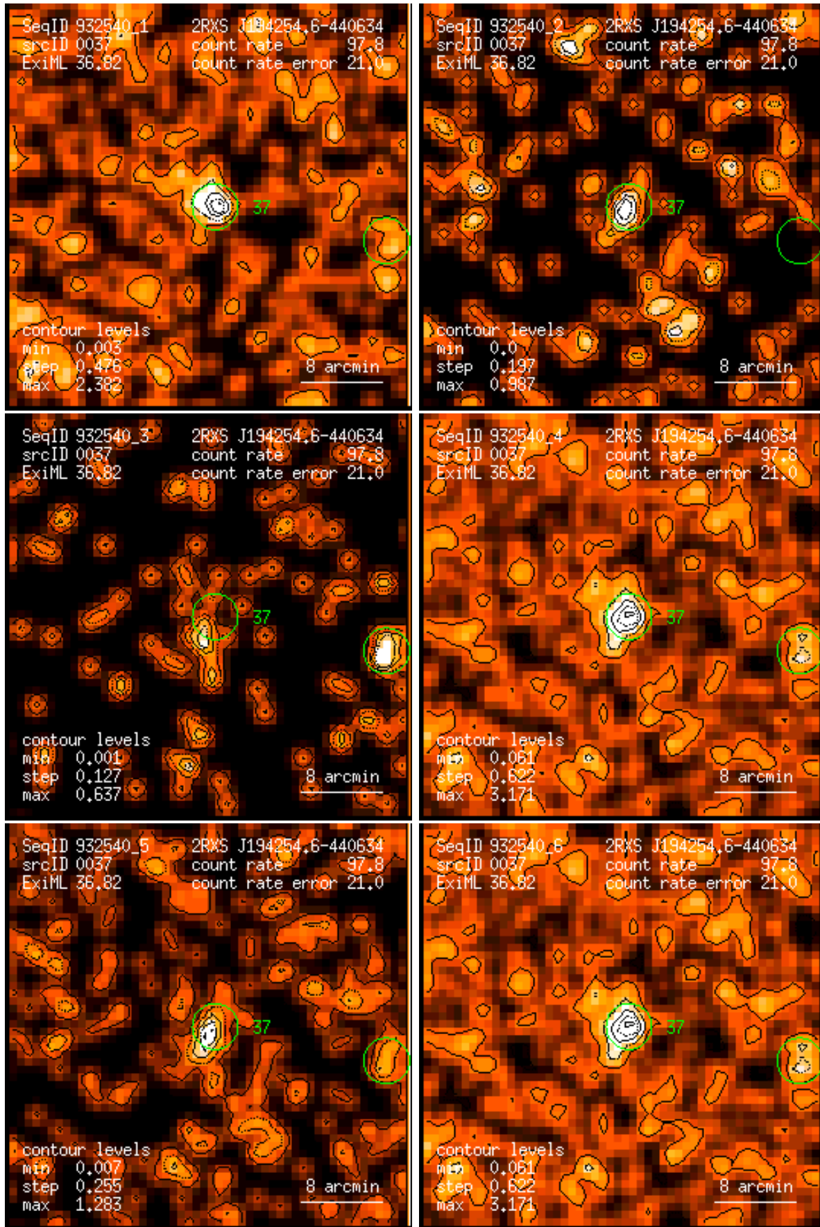
Figure 37: RASS 932540: detection 0037: band rate images, Gaussian filter: (1) PSPC channels 11 – 41, (2) 52 – 90, (3) 91 – 201, (4) 11 – 235, (5) 52 – 201, (6) 11 – 201. Broad band rates in counts/ks. Band rate contour levels in counts/ks/arcmin 2 .
