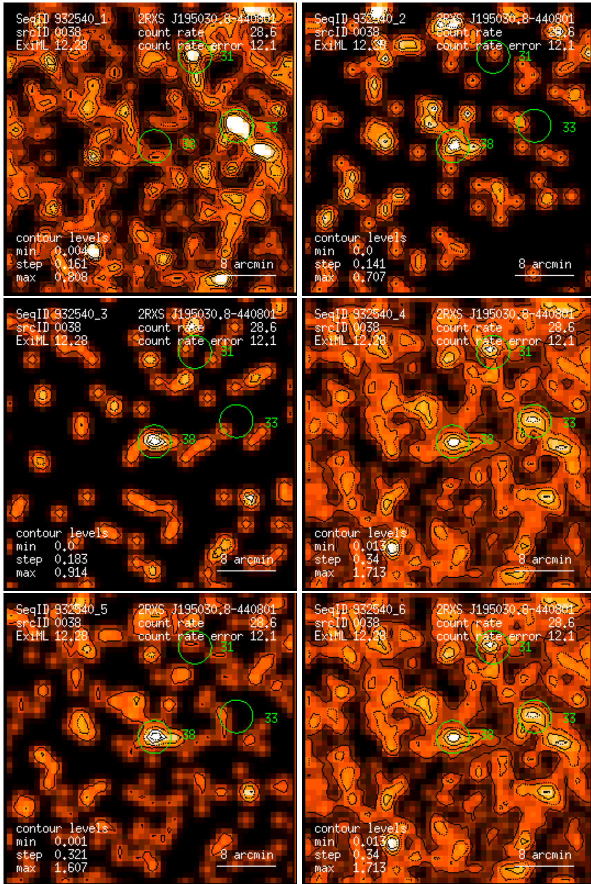
Figure 38: RASS 932540: detection 0038: band rate images, Gaussian filter: (1) PSPC channels 11 – 41, (2) 52 – 90, (3) 91 – 201, (4) 11 – 235, (5) 52 – 201, (6) 11 – 201. Broad band rates in counts/ks. Band rate contour levels in counts/ks/arcmin 2 .
