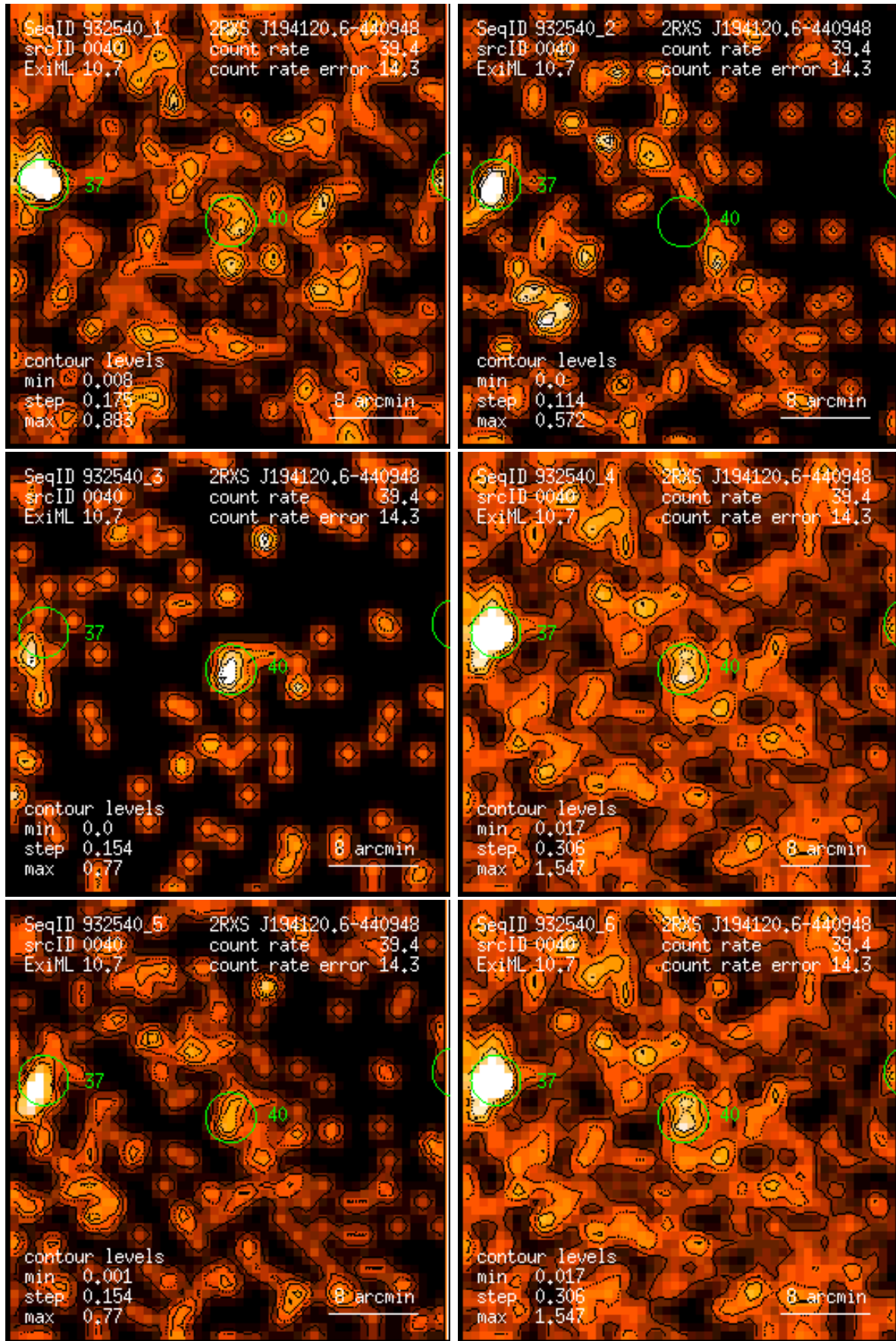
Figure 40: RASS 932540: detection 0040: band rate images, Gaussian filter: (1) PSPC channels 11 – 41, (2) 52 – 90, (3) 91 – 201, (4) 11 – 235, (5) 52 – 201, (6) 11 – 201. Broad band rates in counts/ks. Band rate contour levels in counts/ks/arcmin 2 .
