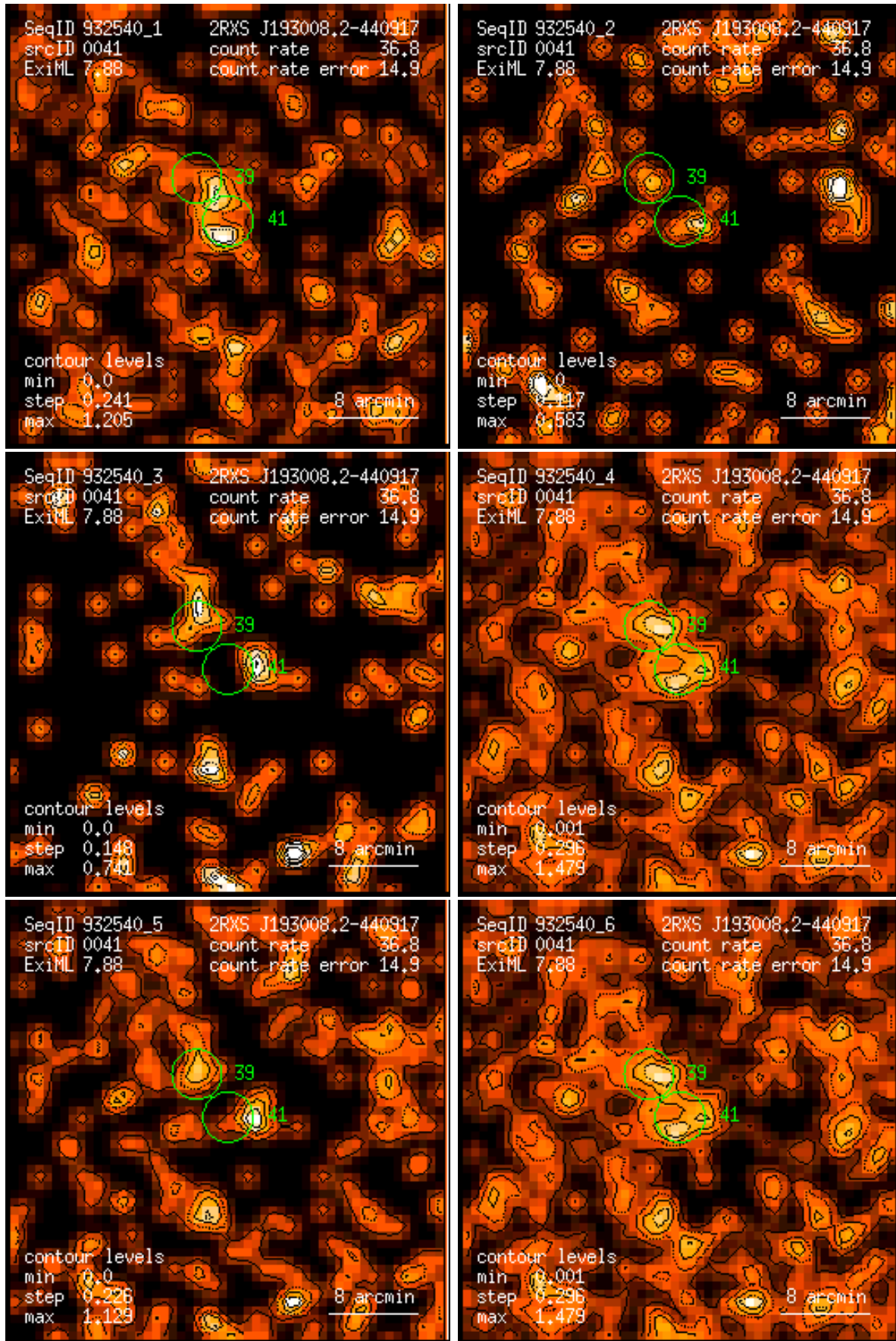
Figure 41: RASS 932540: detection 0041: band rate images, Gaussian filter: (1) PSPC channels 11 – 41, (2) 52 – 90, (3) 91 – 201, (4) 11 – 235, (5) 52 – 201, (6) 11 – 201. Broad band rates in counts/ks. Band rate contour levels in counts/ks/arcmin 2 .
