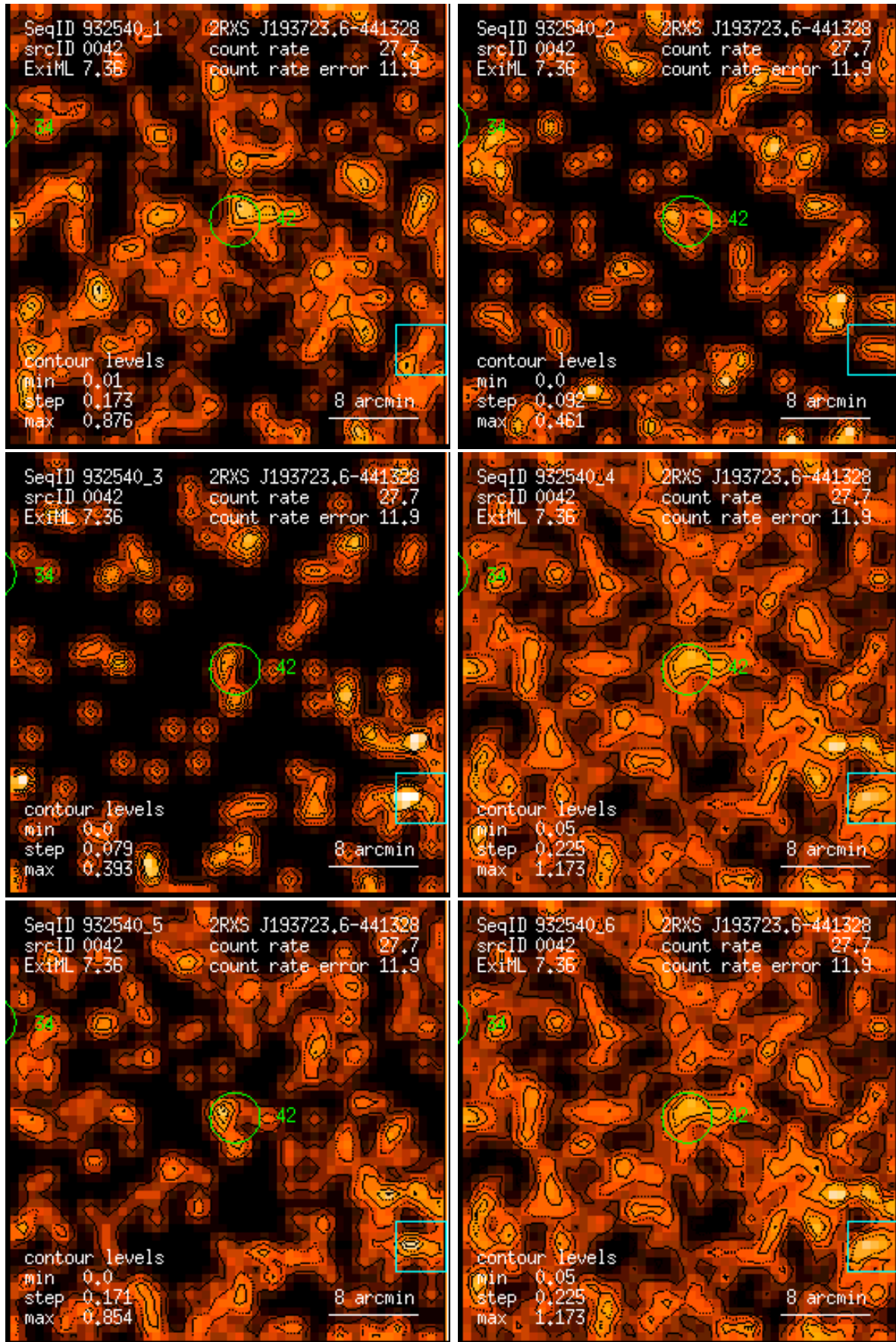
Figure 42: RASS 932540: detection 0042: band rate images, Gaussian filter: (1) PSPC channels 11 – 41, (2) 52 – 90, (3) 91 – 201, (4) 11 – 235, (5) 52 – 201, (6) 11 – 201. Broad band rates in counts/ks. Band rate contour levels in counts/ks/arcmin 2 .
