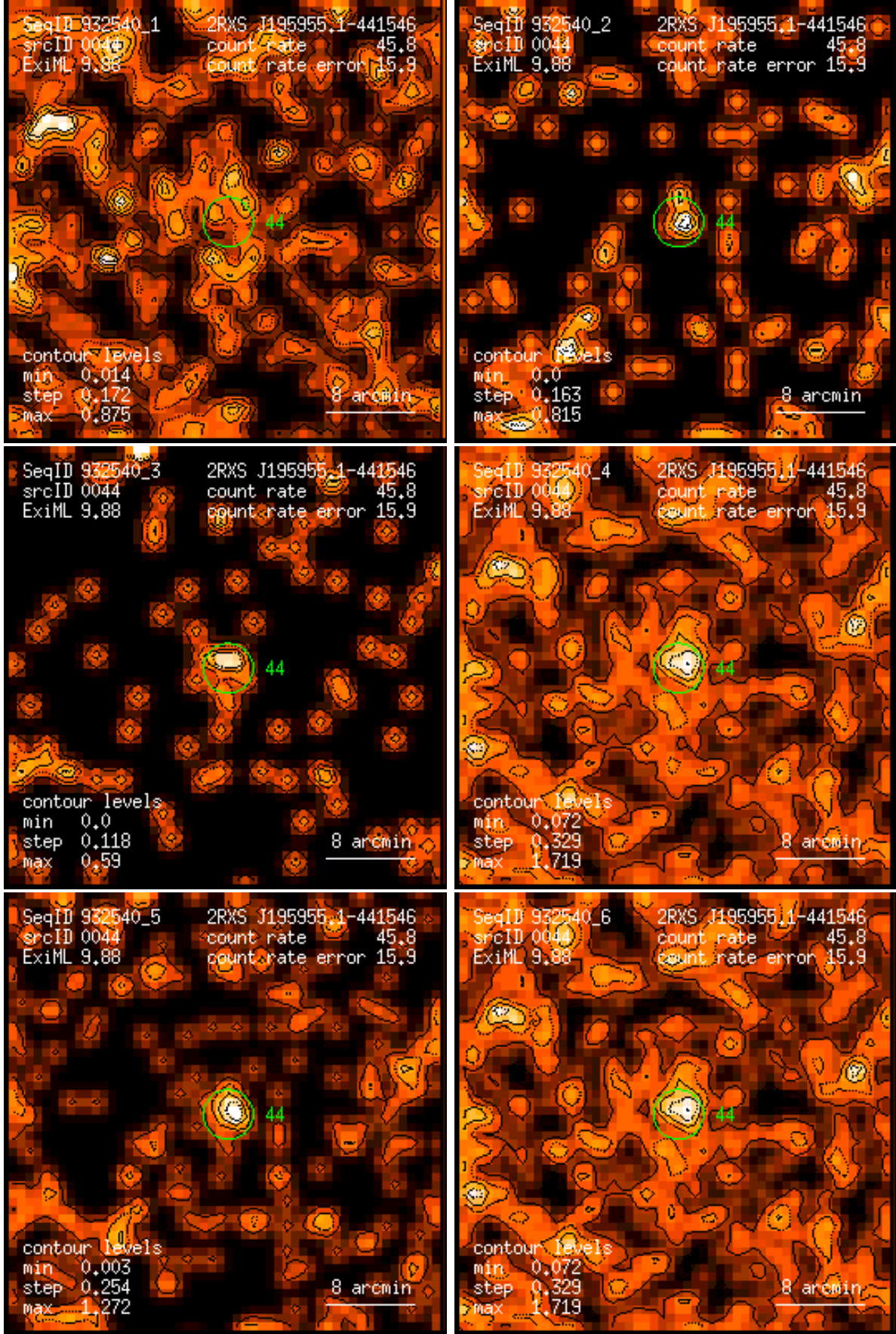
Figure 44: RASS 932540: detection 0044: band rate images, Gaussian filter: (1) PSPC channels 11 – 41, (2) 52 – 90, (3) 91 – 201, (4) 11 – 235, (5) 52 – 201, (6) 11 – 201. Broad band rates in counts/ks. Band rate contour levels in counts/ks/arcmin 2 .
