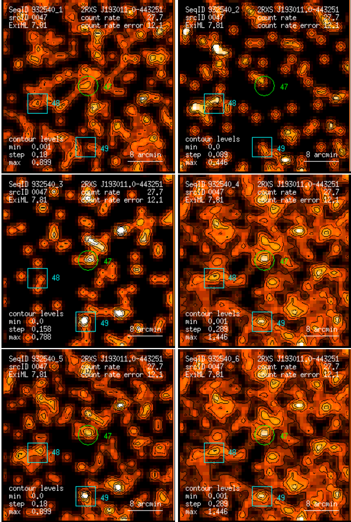
Figure 47: RASS 932540: detection 0047: band rate images, Gaussian filter: (1) PSPC channels 11 – 41, (2) 52 – 90, (3) 91 – 201, (4) 11 – 235, (5) 52 – 201, (6) 11 – 201. Broad band rates in counts/ks. Band rate contour levels in counts/ks/arcmin 2 .
