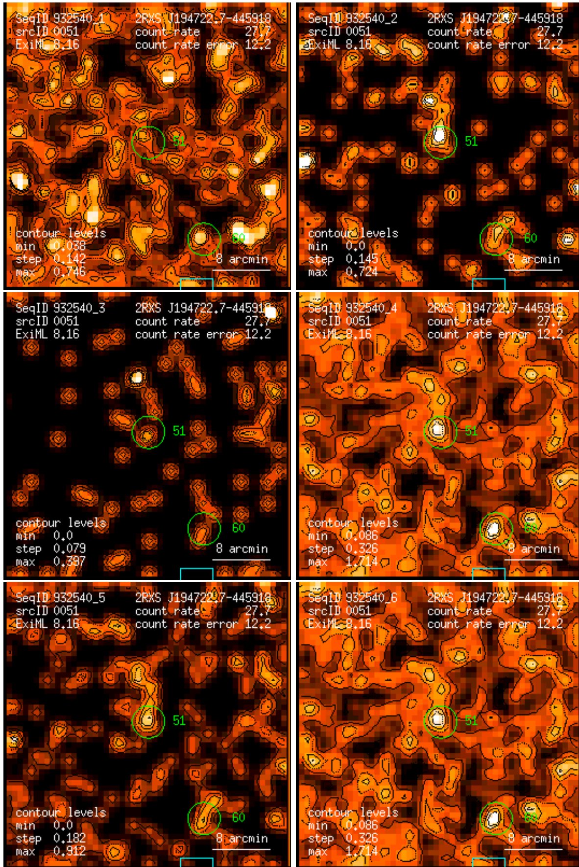
Figure 51: RASS 932540: detection 0051: band rate images, Gaussian filter: (1) PSPC channels 11 – 41, (2) 52 – 90, (3) 91 – 201, (4) 11 – 235, (5) 52 – 201, (6) 11 – 201. Broad band rates in counts/ks. Band rate contour levels in counts/ks/arcmin 2 .
