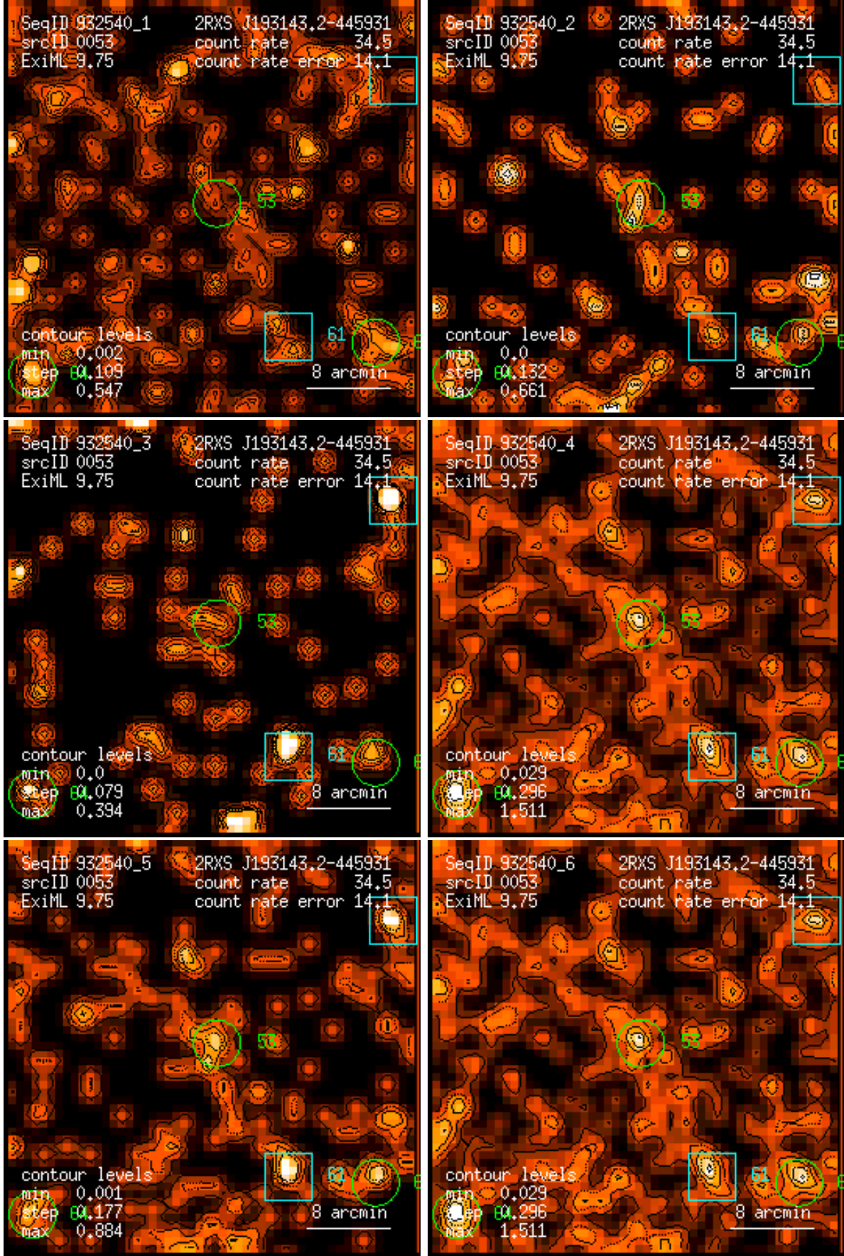
Figure 53: RASS 932540: detection 0053: band rate images, Gaussian filter: (1) PSPC channels 11 – 41, (2) 52 – 90, (3) 91 – 201, (4) 11 – 235, (5) 52 – 201, (6) 11 – 201. Broad band rates in counts/ks. Band rate contour levels in counts/ks/arcmin 2 .
