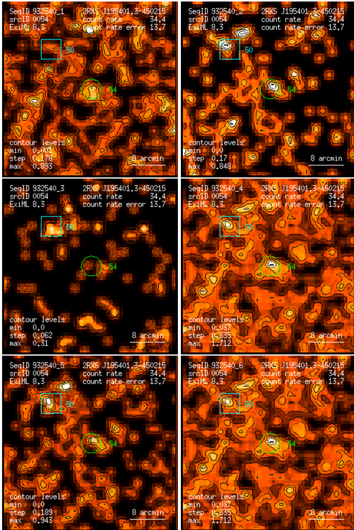
Figure 54: RASS 932540: detection 0054: band rate images, Gaussian filter: (1) PSPC channels 11 – 41, (2) 52 – 90, (3) 91 – 201, (4) 11 – 235, (5) 52 – 201, (6) 11 – 201. Broad band rates in counts/ks. Band rate contour levels in counts/ks/arcmin 2 .
