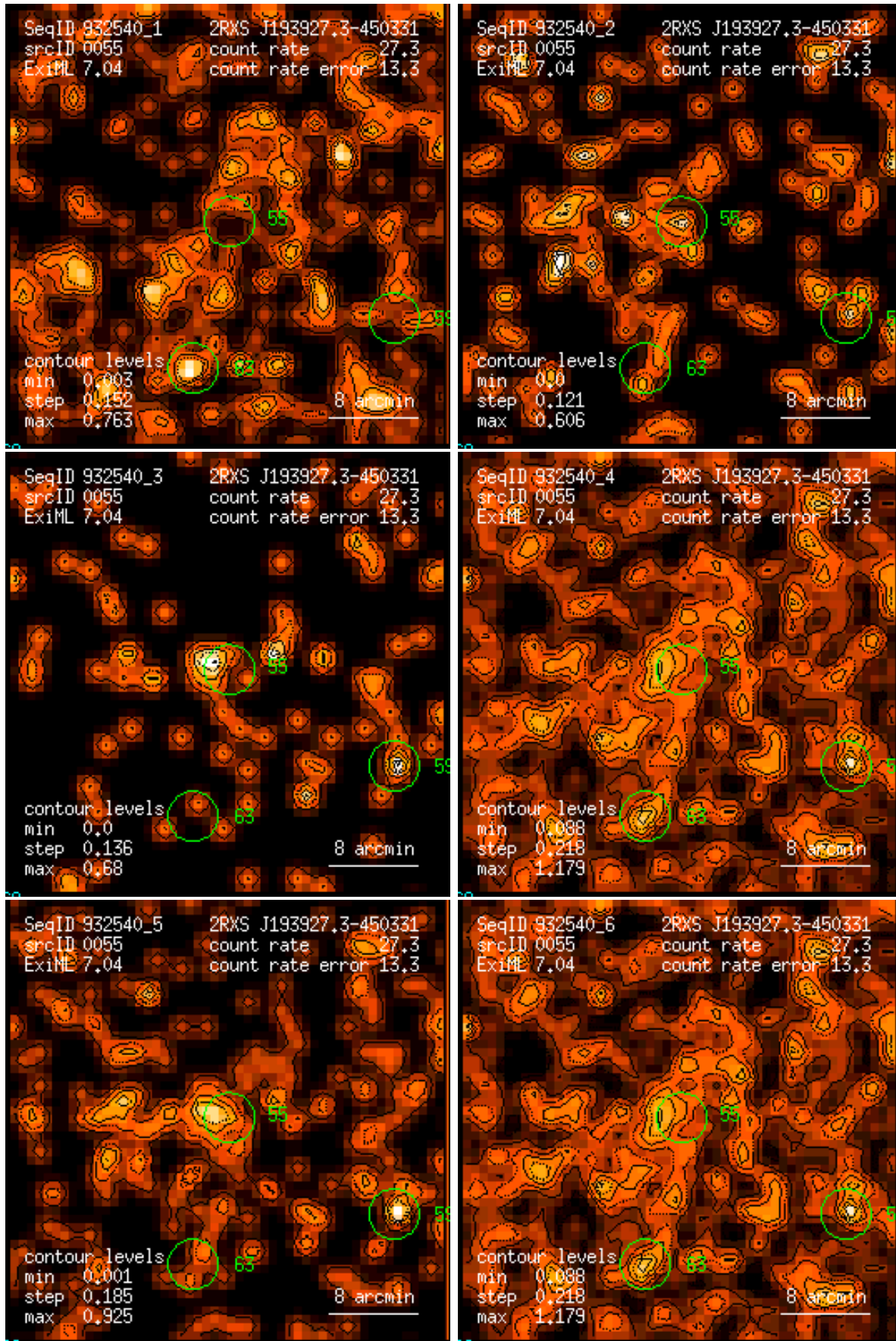
Figure 55: RASS 932540: detection 0055: band rate images, Gaussian filter: (1) PSPC channels 11 – 41, (2) 52 – 90, (3) 91 – 201, (4) 11 – 235, (5) 52 – 201, (6) 11 – 201. Broad band rates in counts/ks. Band rate contour levels in counts/ks/arcmin 2 .
