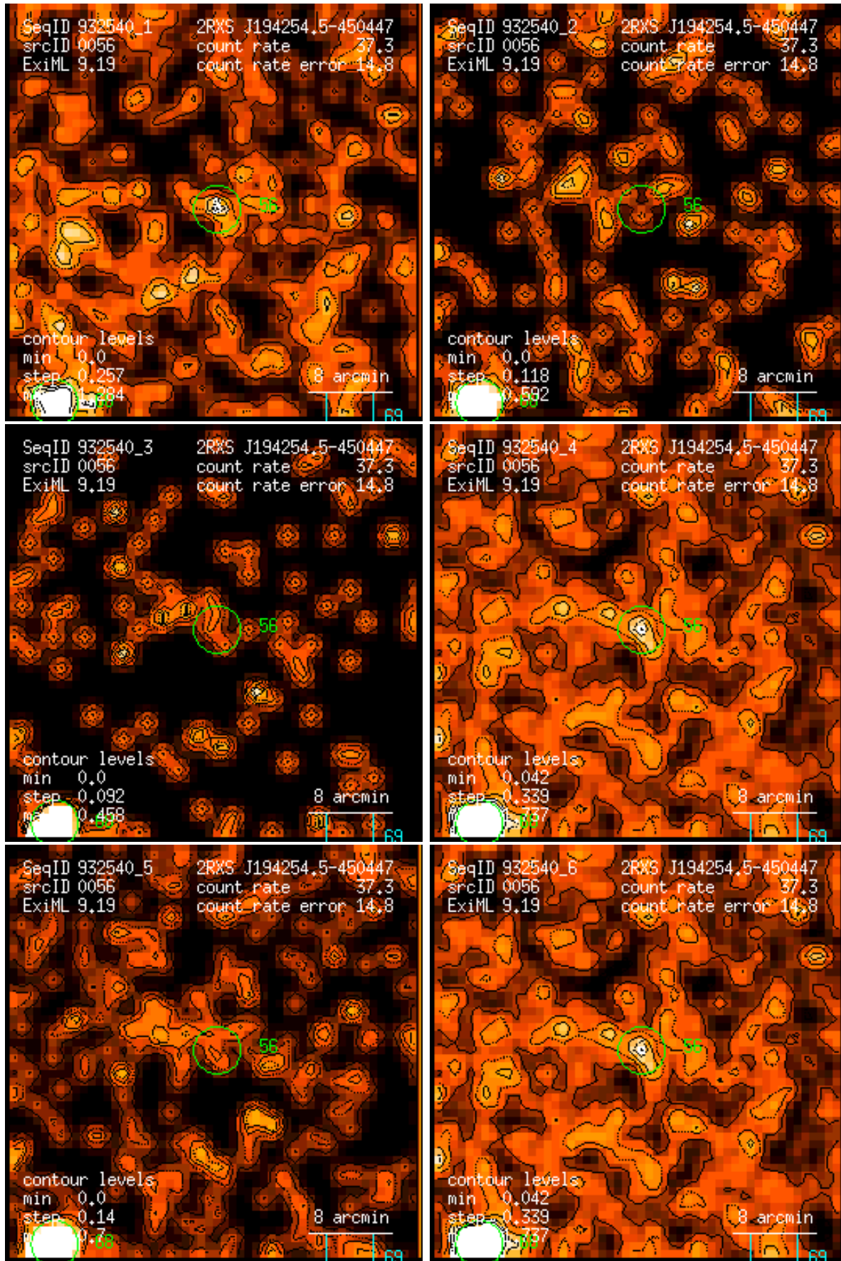
Figure 56: RASS 932540: detection 0056: band rate images, Gaussian filter: (1) PSPC channels 11 – 41, (2) 52 – 90, (3) 91 – 201, (4) 11 – 235, (5) 52 – 201, (6) 11 – 201. Broad band rates in counts/ks. Band rate contour levels in counts/ks/arcmin 2 .
