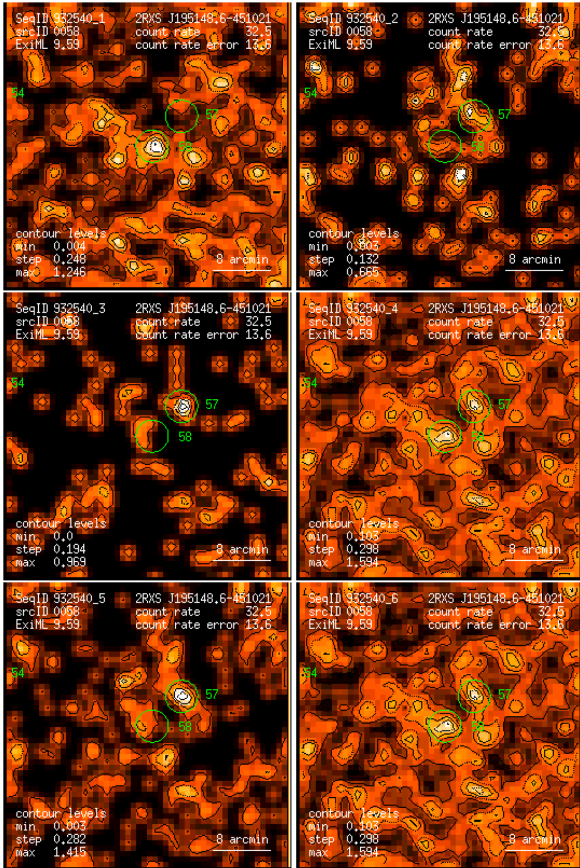
Figure 58: RASS 932540: detection 0058: band rate images, Gaussian filter: (1) PSPC channels 11 – 41, (2) 52 – 90, (3) 91 – 201, (4) 11 – 235, (5) 52 – 201, (6) 11 – 201. Broad band rates in counts/ks. Band rate contour levels in counts/ks/arcmin 2 .
