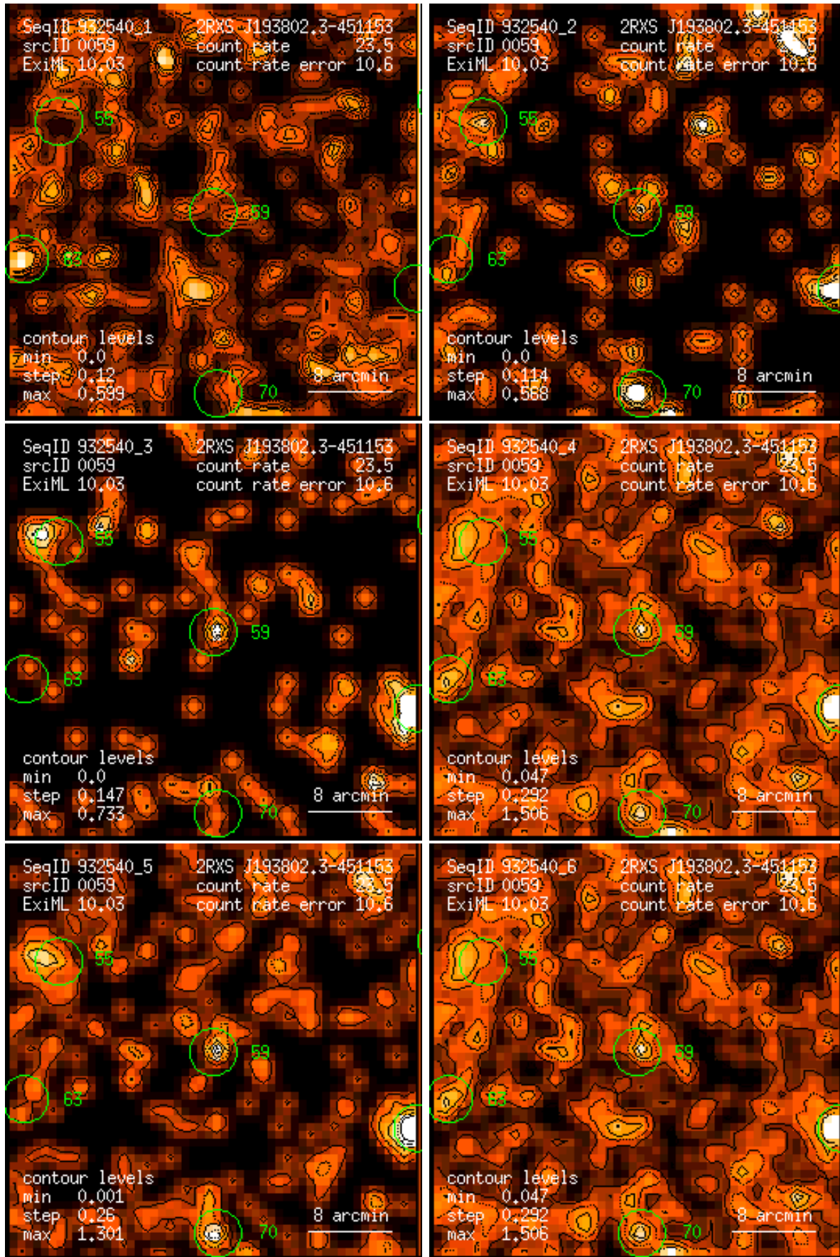
Figure 59: RASS 932540: detection 0059: band rate images, Gaussian filter: (1) PSPC channels 11 – 41, (2) 52 – 90, (3) 91 – 201, (4) 11 – 235, (5) 52 – 201, (6) 11 – 201. Broad band rates in counts/ks. Band rate contour levels in counts/ks/arcmin 2 .
