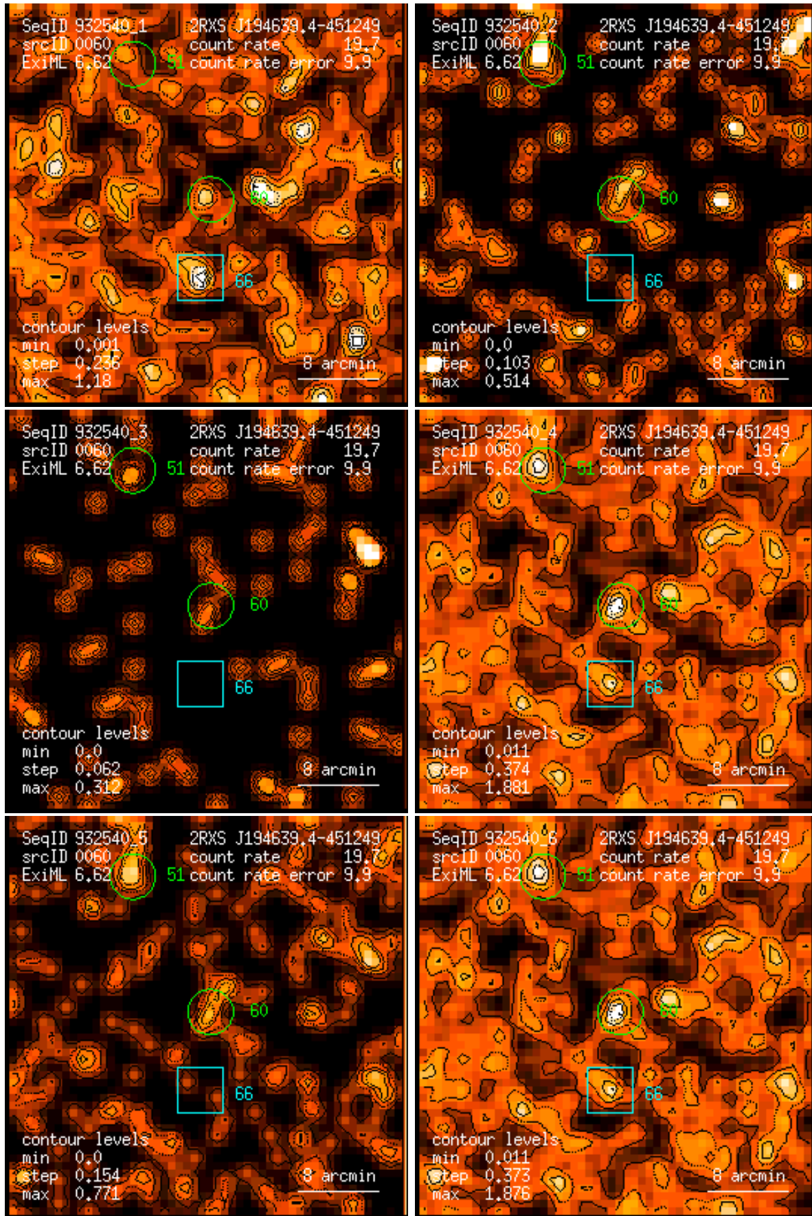
Figure 60: RASS 932540: detection 0060: band rate images, Gaussian filter: (1) PSPC channels 11 – 41, (2) 52 – 90, (3) 91 – 201, (4) 11 – 235, (5) 52 – 201, (6) 11 – 201. Broad band rates in counts/ks. Band rate contour levels in counts/ks/arcmin 2 .
