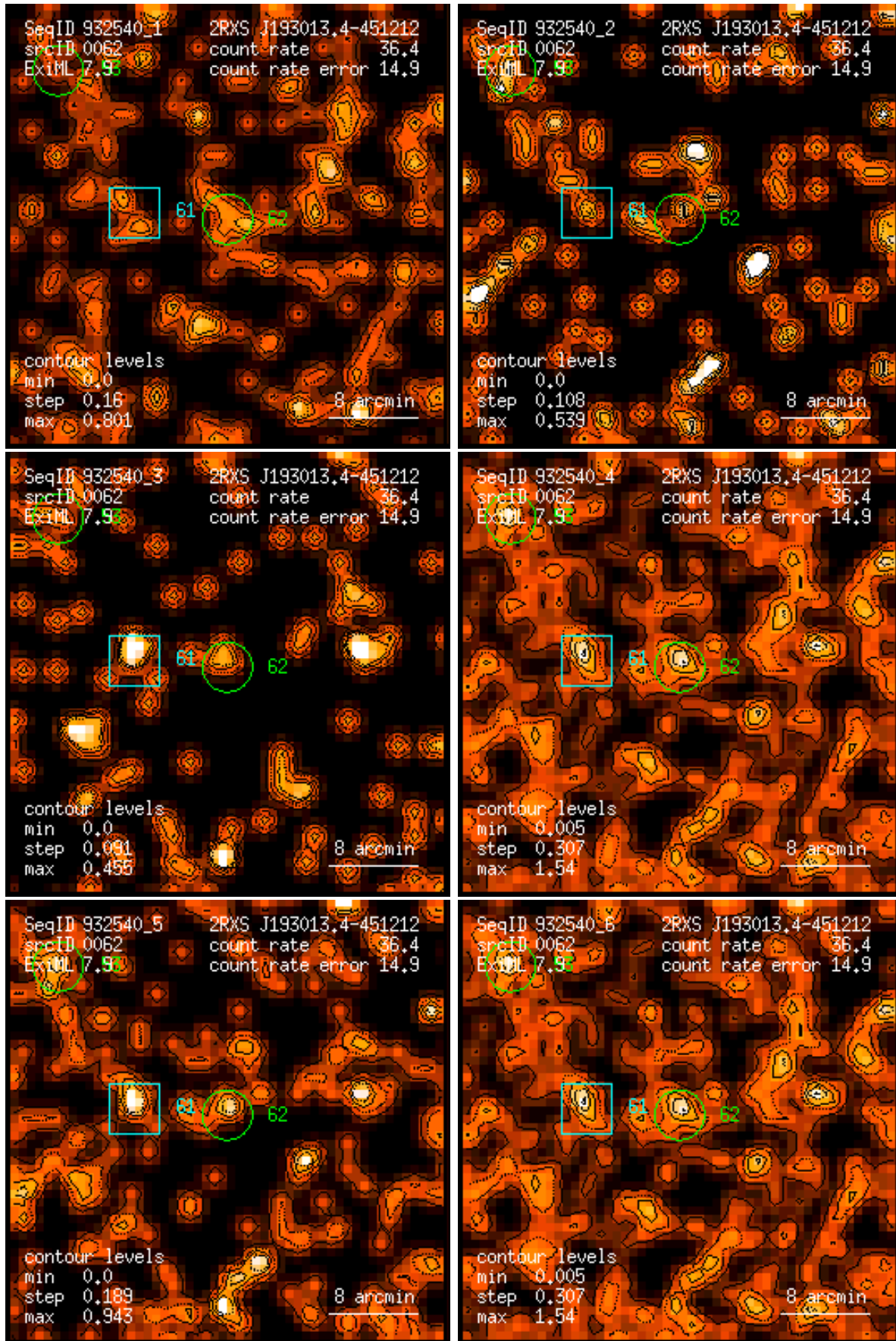
Figure 62: RASS 932540: detection 0062: band rate images, Gaussian filter: (1) PSPC channels 11 – 41, (2) 52 – 90, (3) 91 – 201, (4) 11 – 235, (5) 52 – 201, (6) 11 – 201. Broad band rates in counts/ks. Band rate contour levels in counts/ks/arcmin 2 .
