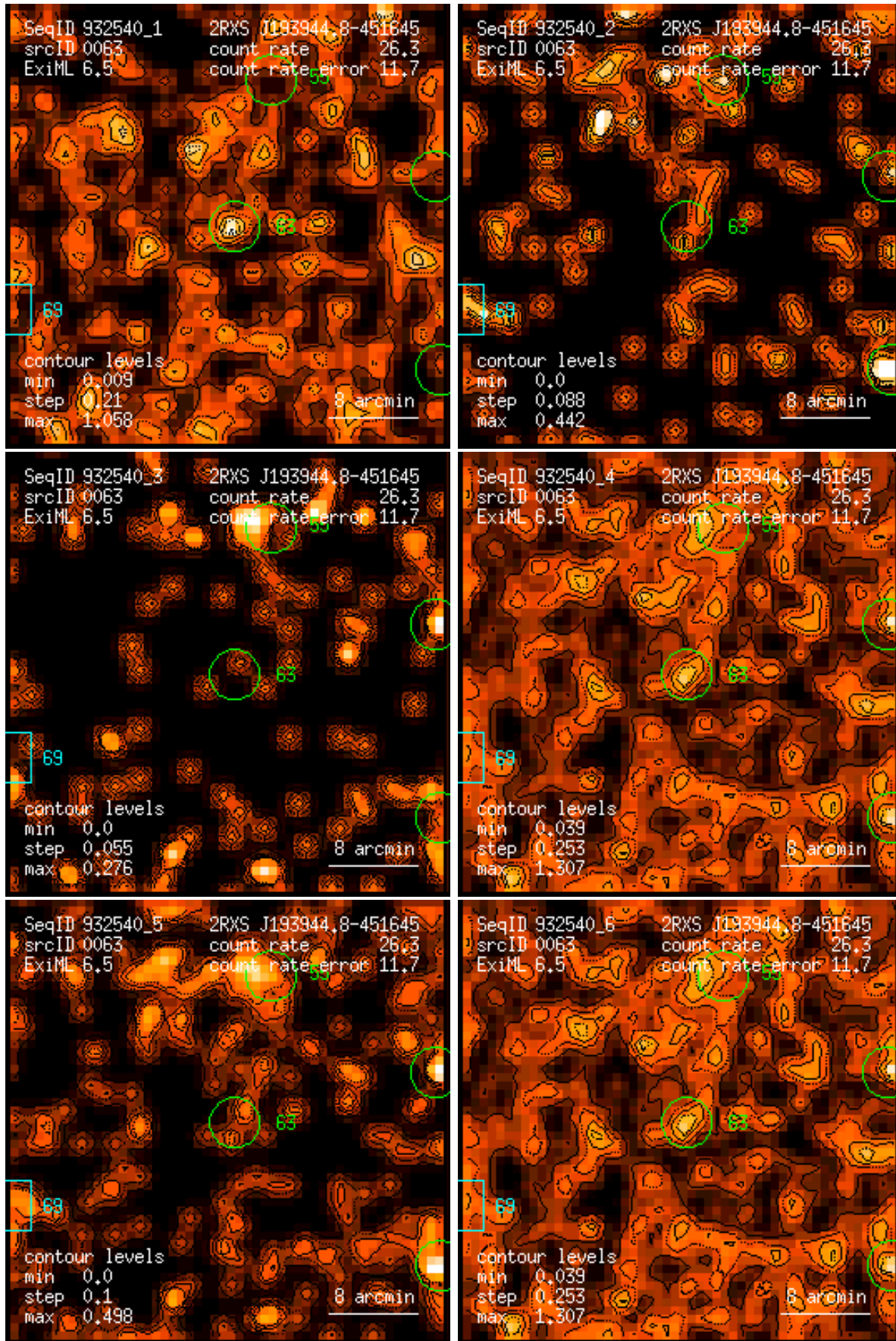
Figure 63: RASS 932540: detection 0063: band rate images, Gaussian filter: (1) PSPC channels 11 – 41, (2) 52 – 90, (3) 91 – 201, (4) 11 – 235, (5) 52 – 201, (6) 11 – 201. Broad band rates in counts/ks. Band rate contour levels in counts/ks/arcmin 2 .
