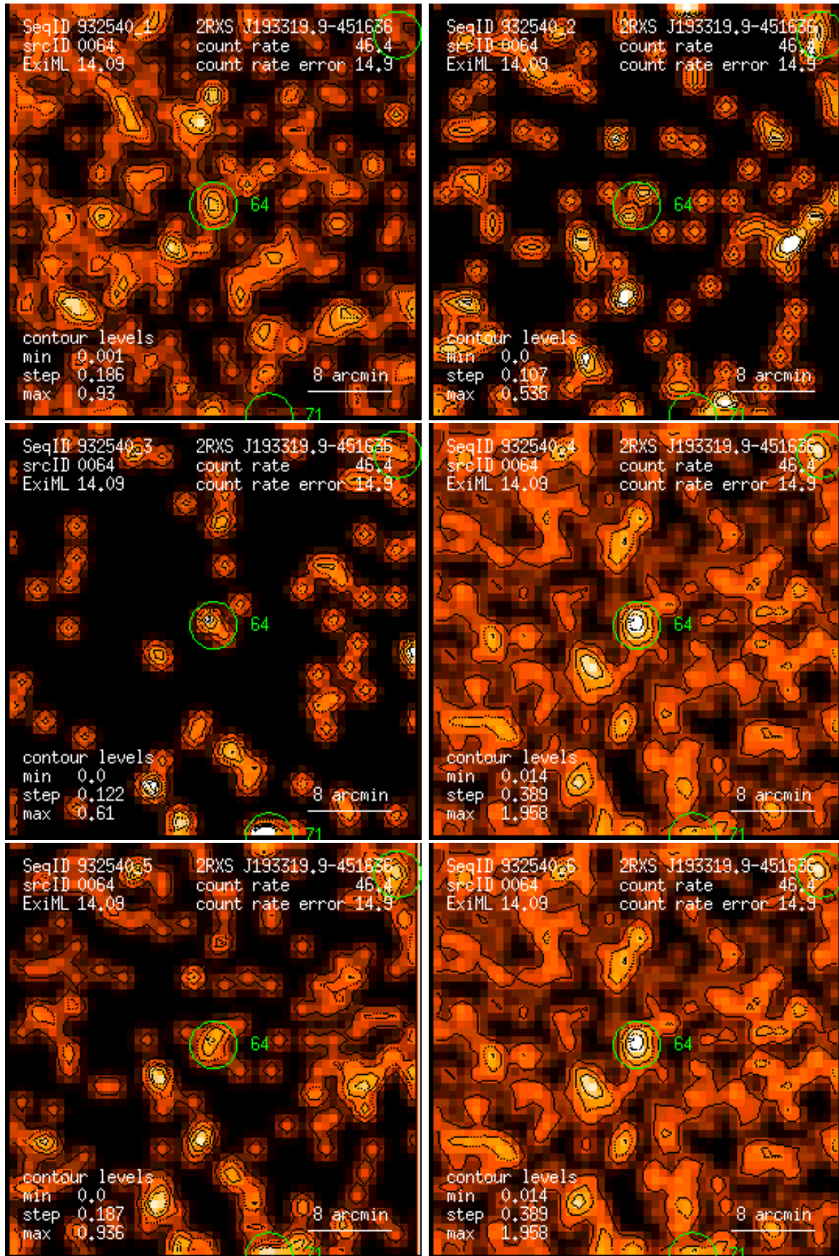
Figure 64: RASS 932540: detection 0064: band rate images, Gaussian filter: (1) PSPC channels 11 – 41, (2) 52 – 90, (3) 91 – 201, (4) 11 – 235, (5) 52 – 201, (6) 11 – 201. Broad band rates in counts/ks. Band rate contour levels in counts/ks/arcmin 2 .
