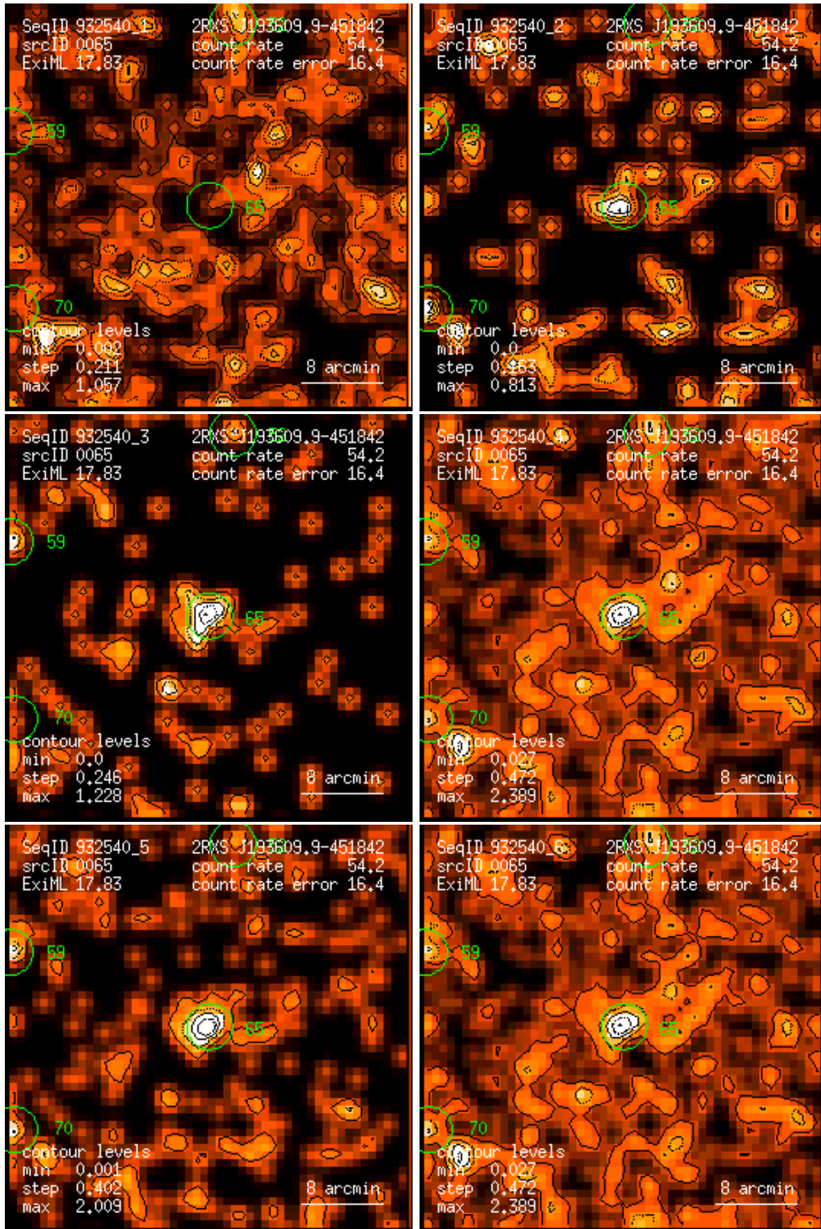
Figure 65: RASS 932540: detection 0065: band rate images, Gaussian filter: (1) PSPC channels 11 – 41, (2) 52 – 90, (3) 91 – 201, (4) 11 – 235, (5) 52 – 201, (6) 11 – 201. Broad band rates in counts/ks. Band rate contour levels in counts/ks/arcmin 2 .
