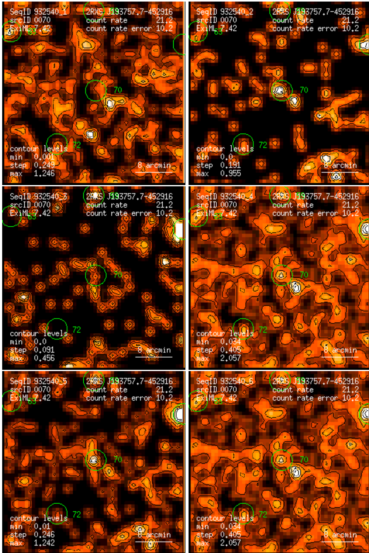
Figure 70: RASS 932540: detection 0070: band rate images, Gaussian filter: (1) PSPC channels 11 – 41, (2) 52 – 90, (3) 91 – 201, (4) 11 – 235, (5) 52 – 201, (6) 11 – 201. Broad band rates in counts/ks. Band rate contour levels in counts/ks/arcmin 2 .
