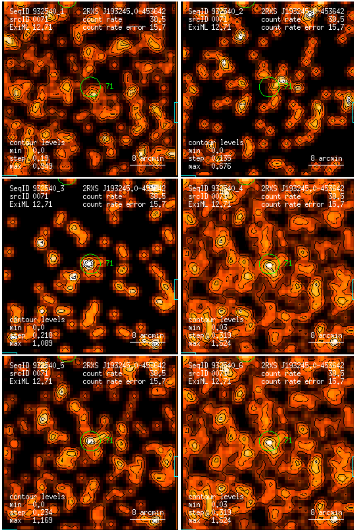
Figure 71: RASS 932540: detection 0071: band rate images, Gaussian filter: (1) PSPC channels 11 – 41, (2) 52 – 90, (3) 91 – 201, (4) 11 – 235, (5) 52 – 201, (6) 11 – 201. Broad band rates in counts/ks. Band rate contour levels in counts/ks/arcmin 2 .
